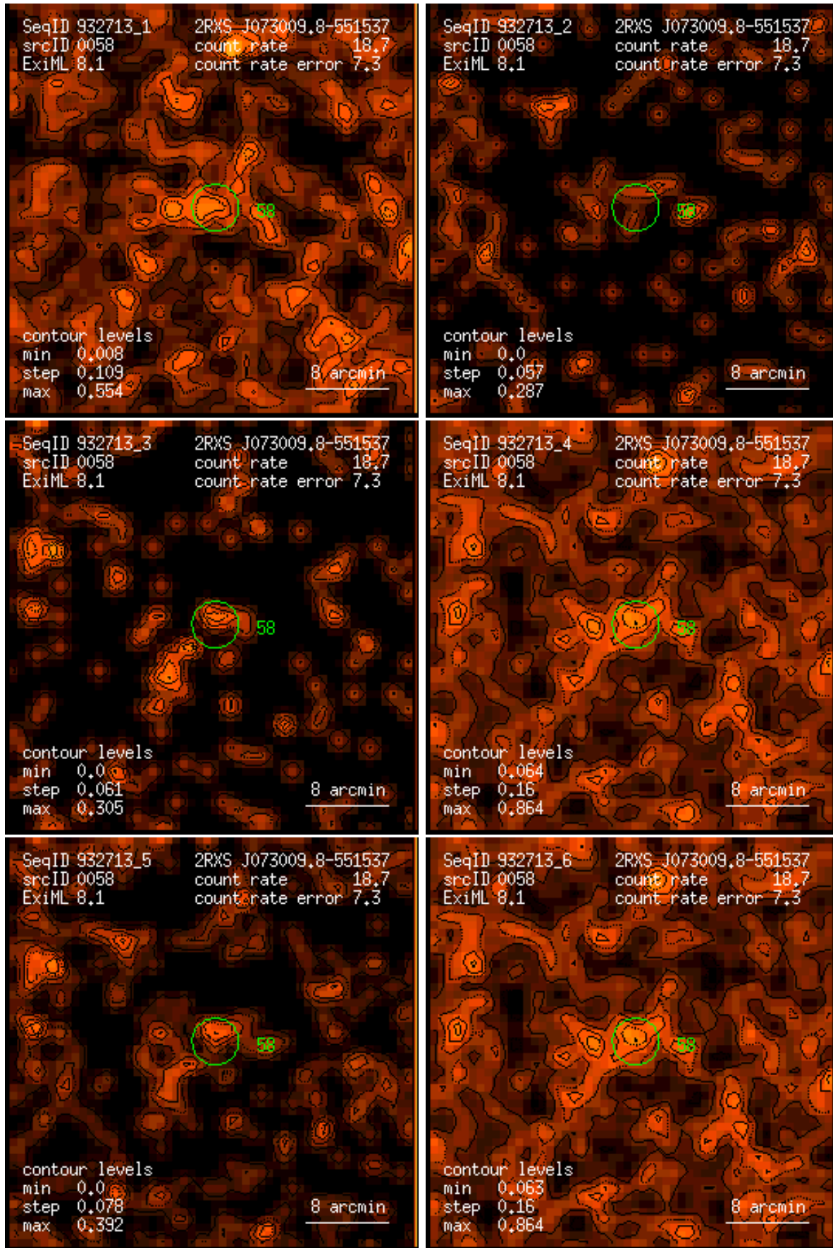
Figure 58: RASS 932713: detection 0058: band rate images, Gaussian filter: (1) PSPC channels 11 – 41, (2) 52 – 90, (3) 91 – 201, (4) 11 – 235, (5) 52 – 201, (6) 11 – 201. Broad band rates in counts/ks. Band rate contour levels in counts/ks/arcmin 2 .
