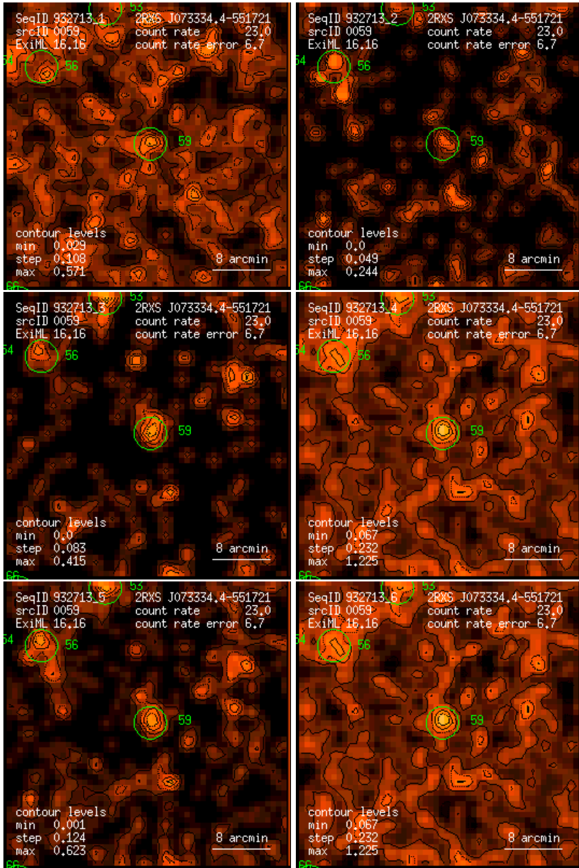
Figure 59: RASS 932713: detection 0059: band rate images, Gaussian filter: (1) PSPC channels 11 – 41, (2) 52 – 90, (3) 91 – 201, (4) 11 – 235, (5) 52 – 201, (6) 11 – 201. Broad band rates in counts/ks. Band rate contour levels in counts/ks/arcmin 2 .
