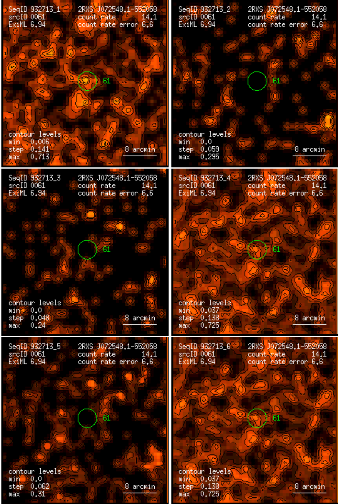
Figure 61: RASS 932713: detection 0061: band rate images, Gaussian filter: (1) PSPC channels 11 – 41, (2) 52 – 90, (3) 91 – 201, (4) 11 – 235, (5) 52 – 201, (6) 11 – 201. Broad band rates in counts/ks. Band rate contour levels in counts/ks/arcmin 2 .
