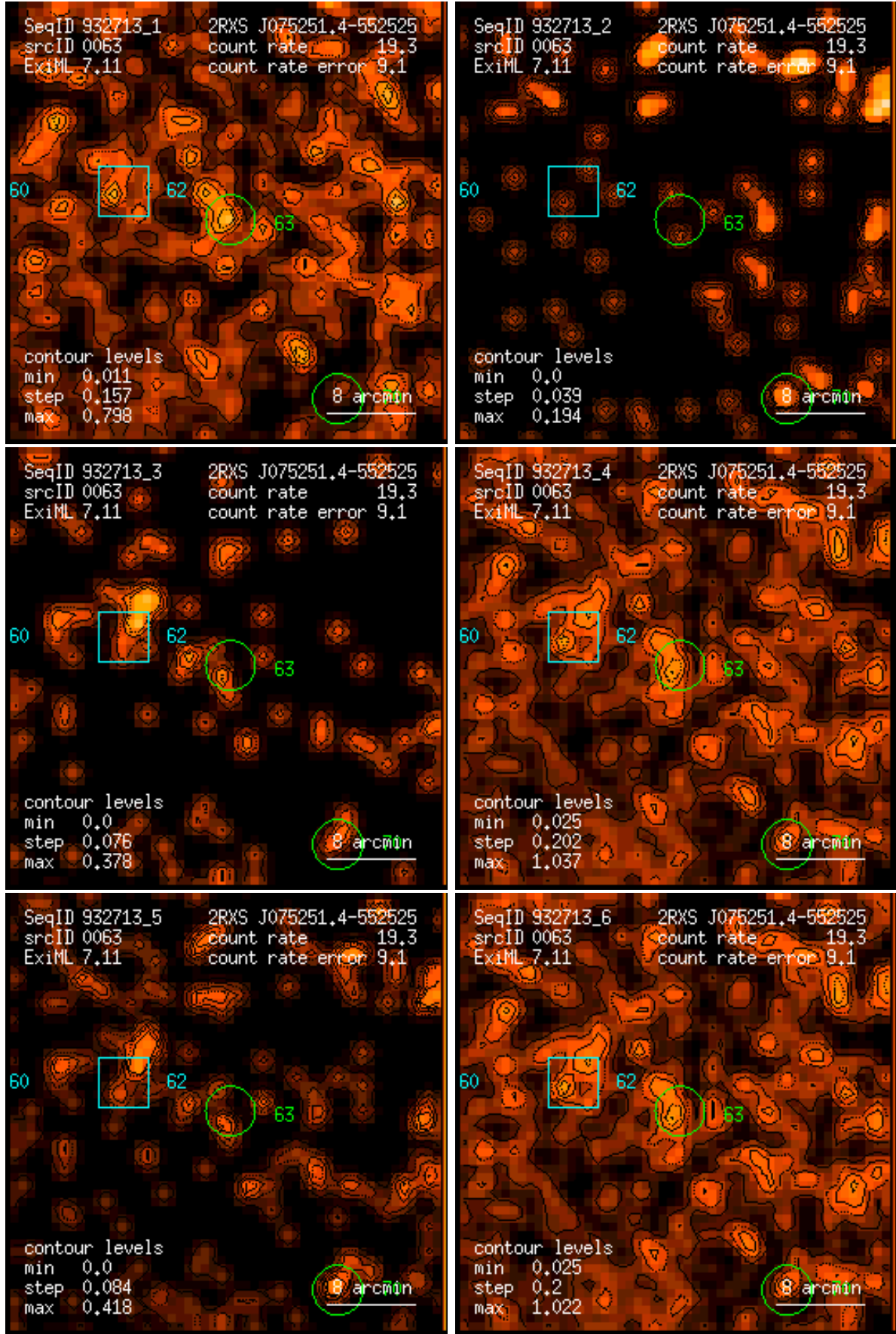
Figure 63: RASS 932713: detection 0063: band rate images, Gaussian filter: (1) PSPC channels 11 – 41, (2) 52 – 90, (3) 91 – 201, (4) 11 – 235, (5) 52 – 201, (6) 11 – 201. Broad band rates in counts/ks. Band rate contour levels in counts/ks/arcmin 2 .
