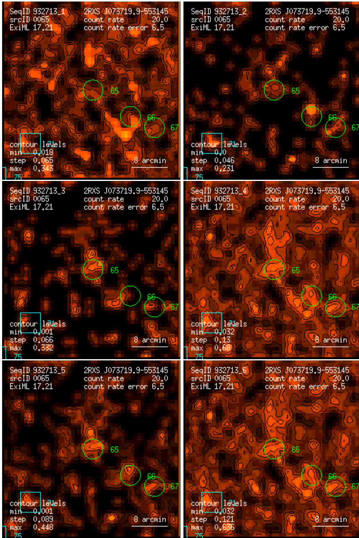
Figure 65: RASS 932713: detection 0065: band rate images, Gaussian filter: (1) PSPC channels 11 – 41, (2) 52 – 90, (3) 91 – 201, (4) 11 – 235, (5) 52 – 201, (6) 11 – 201. Broad band rates in counts/ks. Band rate contour levels in counts/ks/arcmin 2 .
