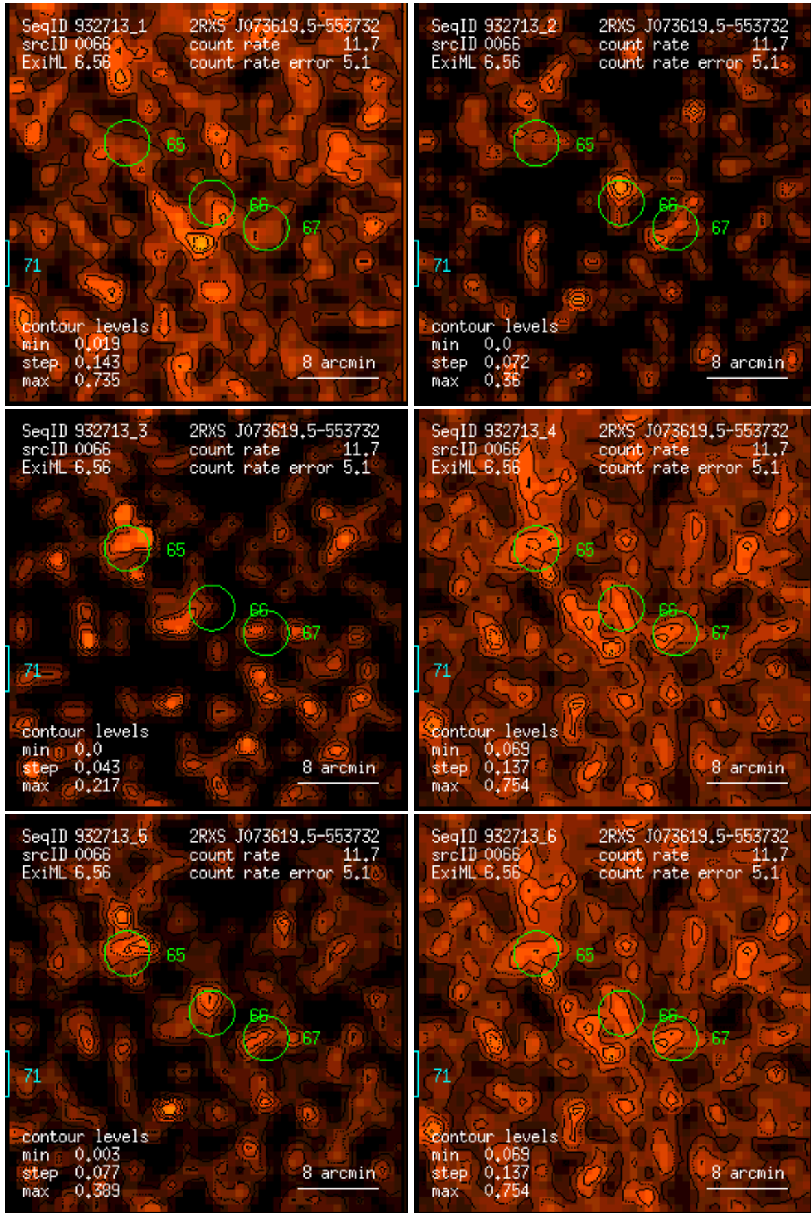
Figure 66: RASS 932713: detection 0066: band rate images, Gaussian filter: (1) PSPC channels 11 – 41, (2) 52 – 90, (3) 91 – 201, (4) 11 – 235, (5) 52 – 201, (6) 11 – 201. Broad band rates in counts/ks. Band rate contour levels in counts/ks/arcmin 2 .
