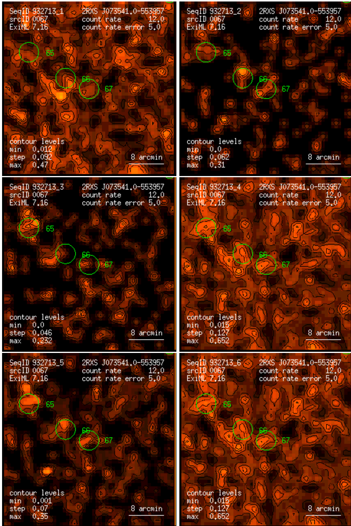
Figure 67: RASS 932713: detection 0067: band rate images, Gaussian filter: (1) PSPC channels 11 – 41, (2) 52 – 90, (3) 91 – 201, (4) 11 – 235, (5) 52 – 201, (6) 11 – 201. Broad band rates in counts/ks. Band rate contour levels in counts/ks/arcmin 2 .
