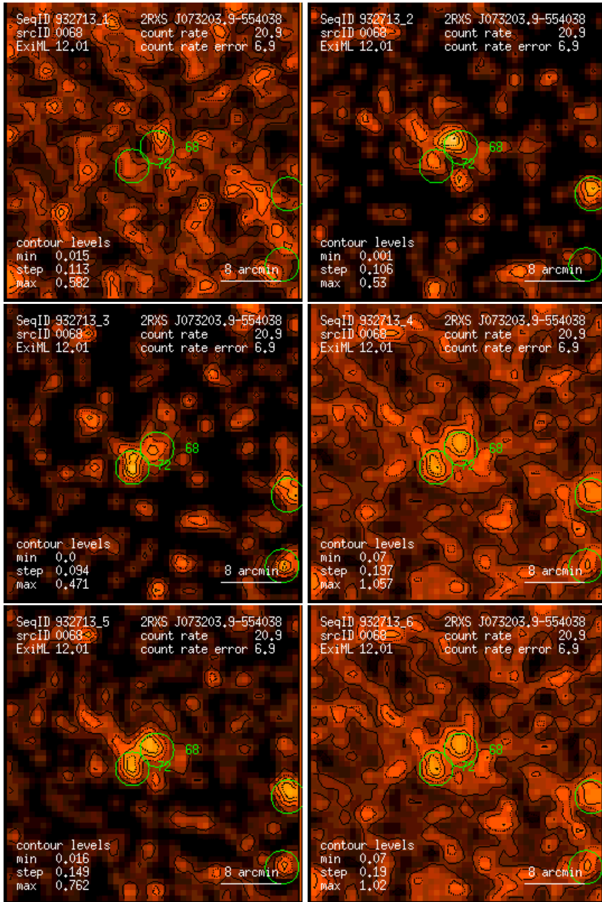
Figure 68: RASS 932713: detection 0068: band rate images, Gaussian filter: (1) PSPC channels 11 – 41, (2) 52 – 90, (3) 91 – 201, (4) 11 – 235, (5) 52 – 201, (6) 11 – 201. Broad band rates in counts/ks. Band rate contour levels in counts/ks/arcmin 2 .
