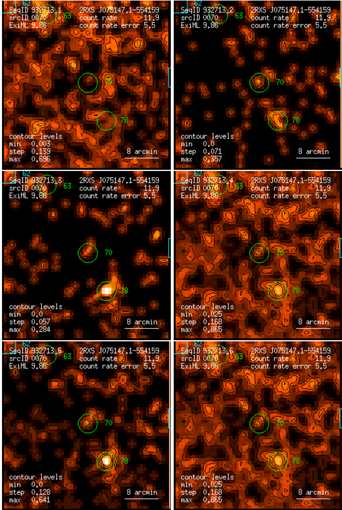
Figure 70: RASS 932713: detection 0070: band rate images, Gaussian filter: (1) PSPC channels 11 – 41, (2) 52 – 90, (3) 91 – 201, (4) 11 – 235, (5) 52 – 201, (6) 11 – 201. Broad band rates in counts/ks. Band rate contour levels in counts/ks/arcmin 2 .
