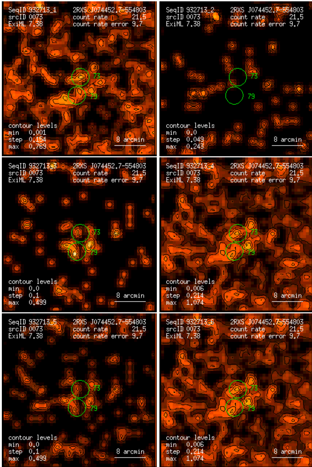
Figure 73: RASS 932713: detection 0073: band rate images, Gaussian filter: (1) PSPC channels 11 – 41, (2) 52 – 90, (3) 91 – 201, (4) 11 – 235, (5) 52 – 201, (6) 11 – 201. Broad band rates in counts/ks. Band rate contour levels in counts/ks/arcmin 2 .
