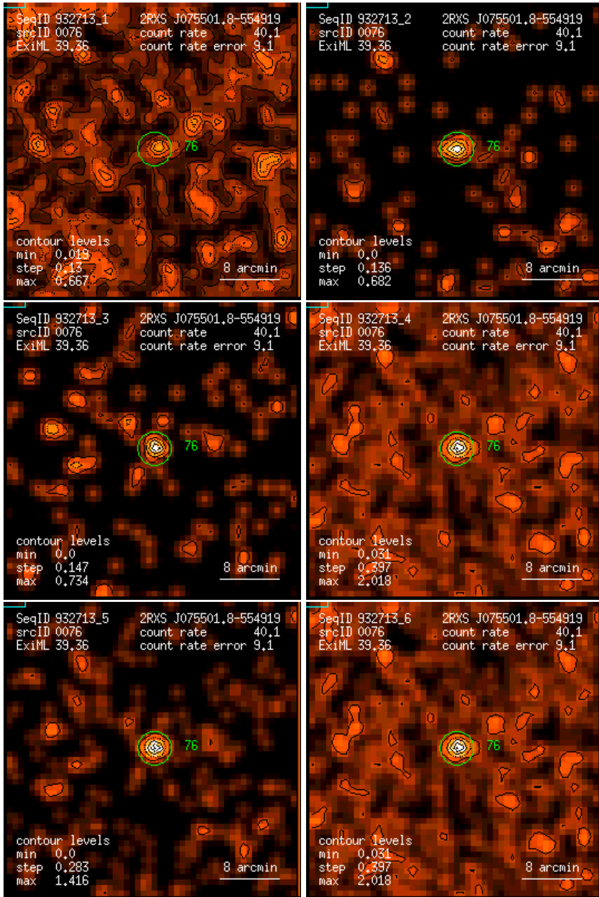
Figure 76: RASS 932713: detection 0076: band rate images, Gaussian filter: (1) PSPC channels 11 – 41, (2) 52 – 90, (3) 91 – 201, (4) 11 – 235, (5) 52 – 201, (6) 11 – 201. Broad band rates in counts/ks. Band rate contour levels in counts/ks/arcmin 2 .
