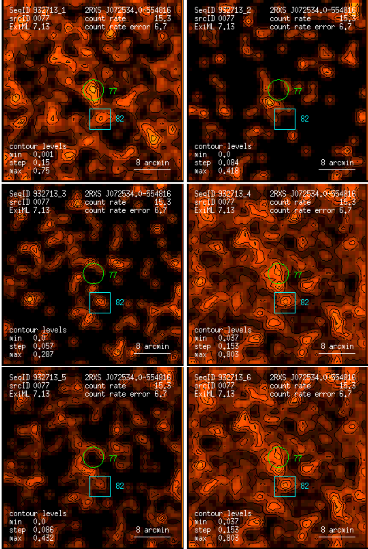
Figure 77: RASS 932713: detection 0077: band rate images, Gaussian filter: (1) PSPC channels 11 – 41, (2) 52 – 90, (3) 91 – 201, (4) 11 – 235, (5) 52 – 201, (6) 11 – 201. Broad band rates in counts/ks. Band rate contour levels in counts/ks/arcmin 2 .
