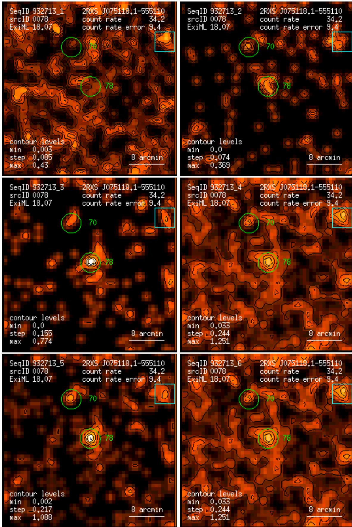
Figure 78: RASS 932713: detection 0078: band rate images, Gaussian filter: (1) PSPC channels 11 – 41, (2) 52 – 90, (3) 91 – 201, (4) 11 – 235, (5) 52 – 201, (6) 11 – 201. Broad band rates in counts/ks. Band rate contour levels in counts/ks/arcmin 2 .
