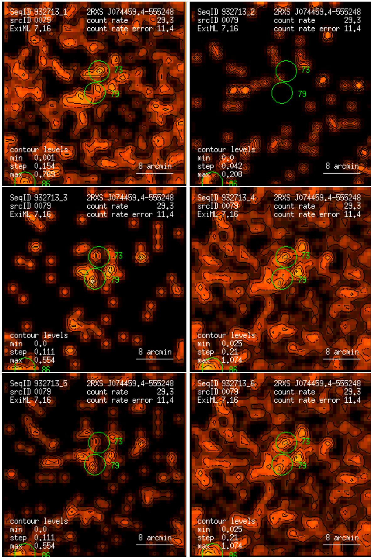
Figure 79: RASS 932713: detection 0079: band rate images, Gaussian filter: (1) PSPC channels 11 – 41, (2) 52 – 90, (3) 91 – 201, (4) 11 – 235, (5) 52 – 201, (6) 11 – 201. Broad band rates in counts/ks. Band rate contour levels in counts/ks/arcmin 2 .
