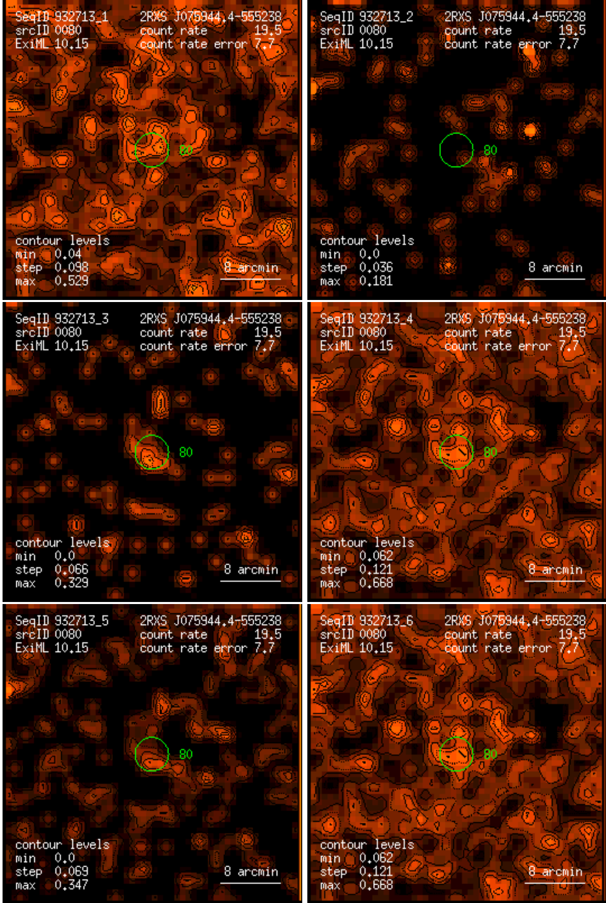
Figure 80: RASS 932713: detection 0080: band rate images, Gaussian filter: (1) PSPC channels 11 – 41, (2) 52 – 90, (3) 91 – 201, (4) 11 – 235, (5) 52 – 201, (6) 11 – 201. Broad band rates in counts/ks. Band rate contour levels in counts/ks/arcmin 2 .
