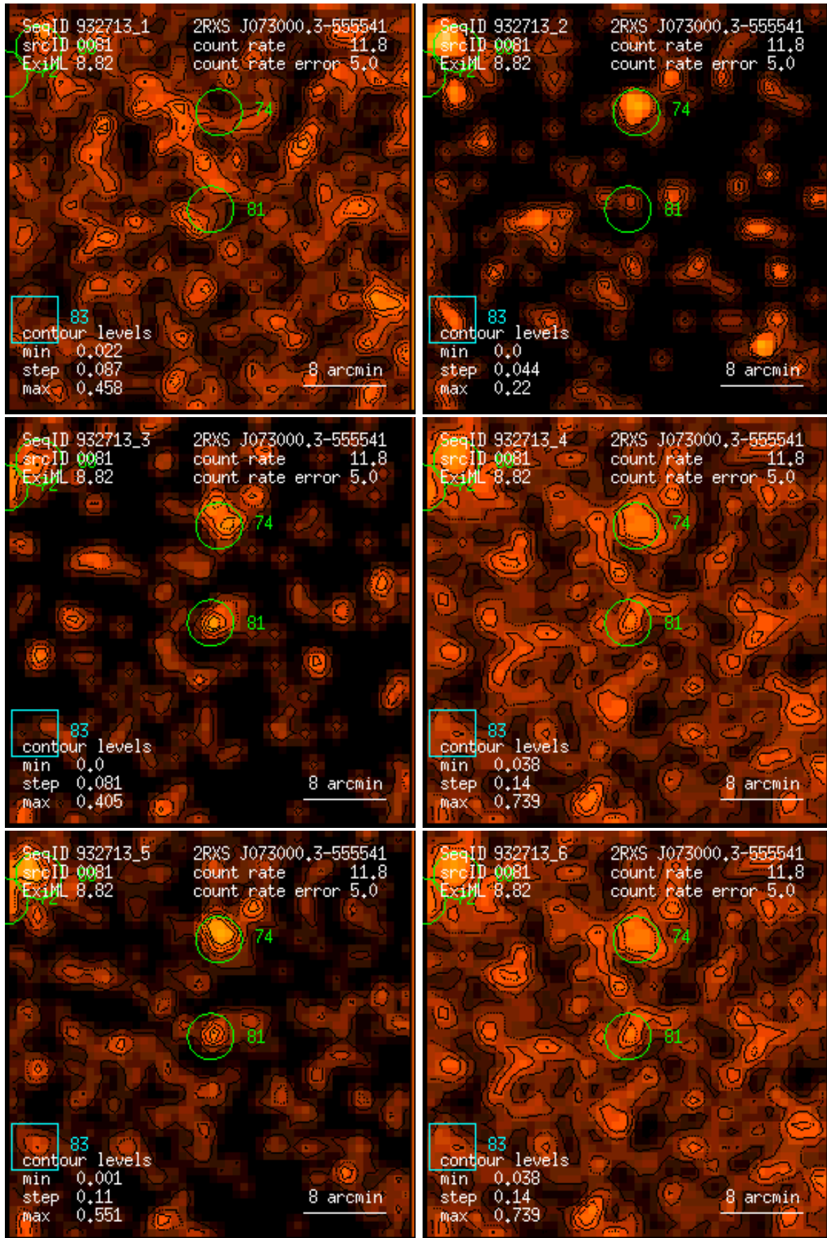
Figure 81: RASS 932713: detection 0081: band rate images, Gaussian filter: (1) PSPC channels 11 – 41, (2) 52 – 90, (3) 91 – 201, (4) 11 – 235, (5) 52 – 201, (6) 11 – 201. Broad band rates in counts/ks. Band rate contour levels in counts/ks/arcmin 2 .
