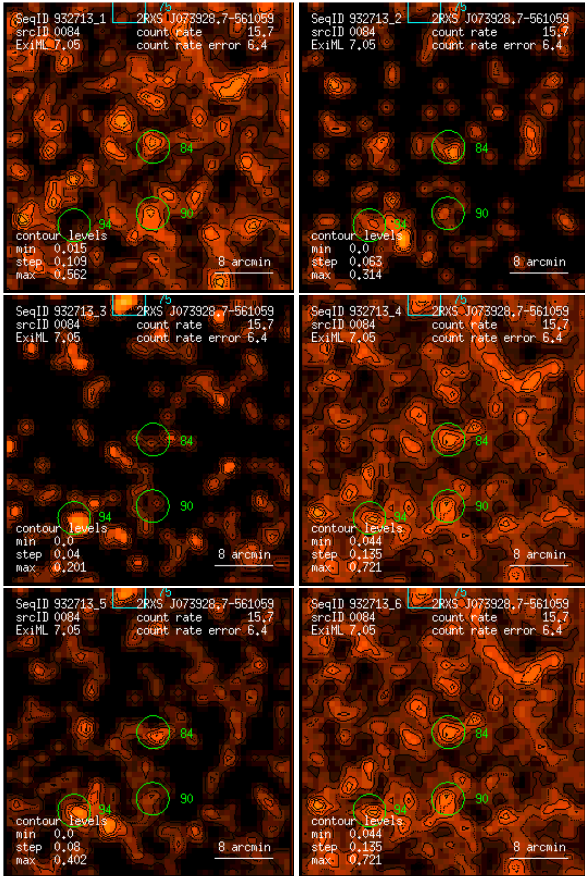
Figure 84: RASS 932713: detection 0084: band rate images, Gaussian filter: (1) PSPC channels 11 – 41, (2) 52 – 90, (3) 91 – 201, (4) 11 – 235, (5) 52 – 201, (6) 11 – 201. Broad band rates in counts/ks. Band rate contour levels in counts/ks/arcmin 2 .
