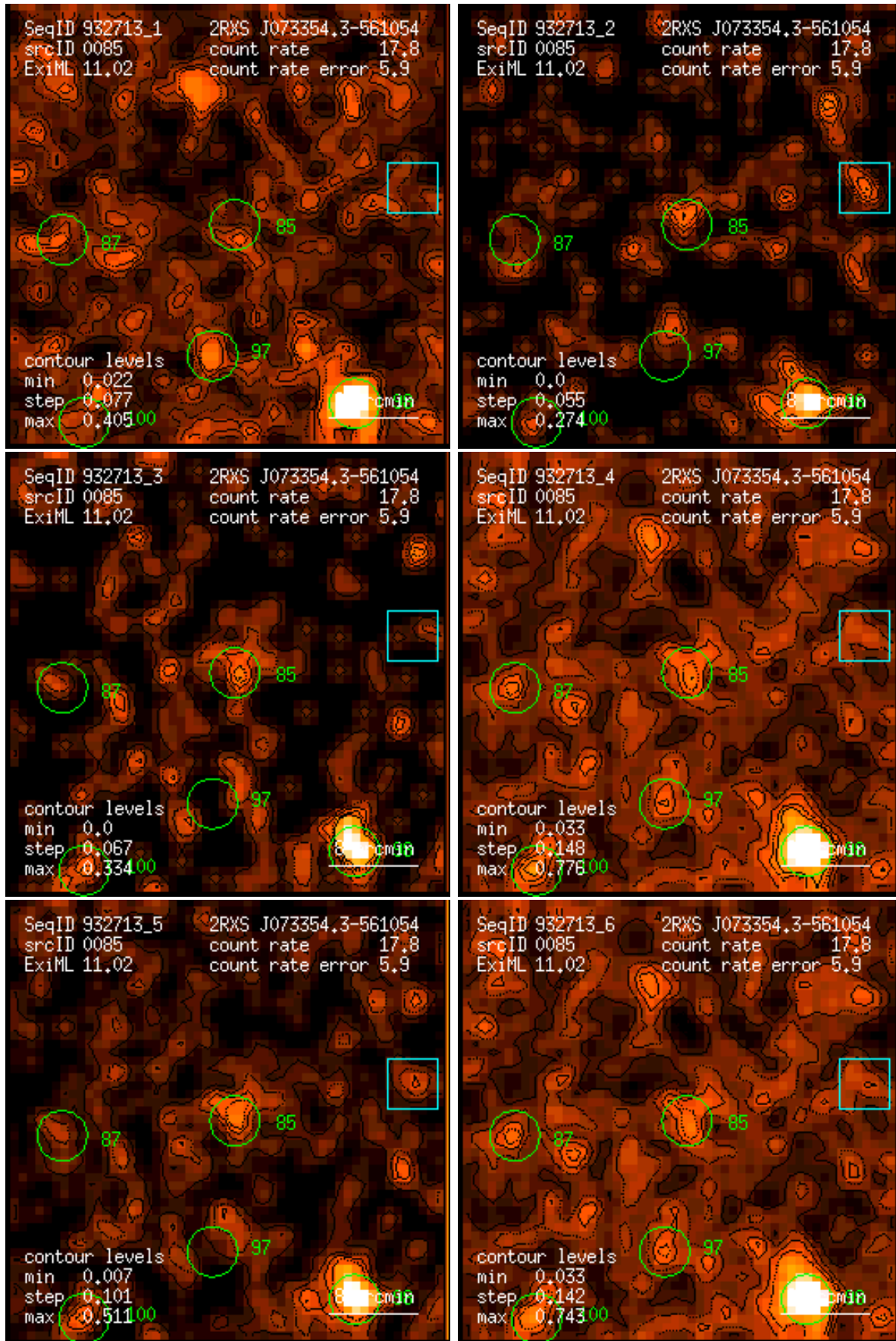
Figure 85: RASS 932713: detection 0085: band rate images, Gaussian filter: (1) PSPC channels 11 – 41, (2) 52 – 90, (3) 91 – 201, (4) 11 – 235, (5) 52 – 201, (6) 11 – 201. Broad band rates in counts/ks. Band rate contour levels in counts/ks/arcmin 2 .
