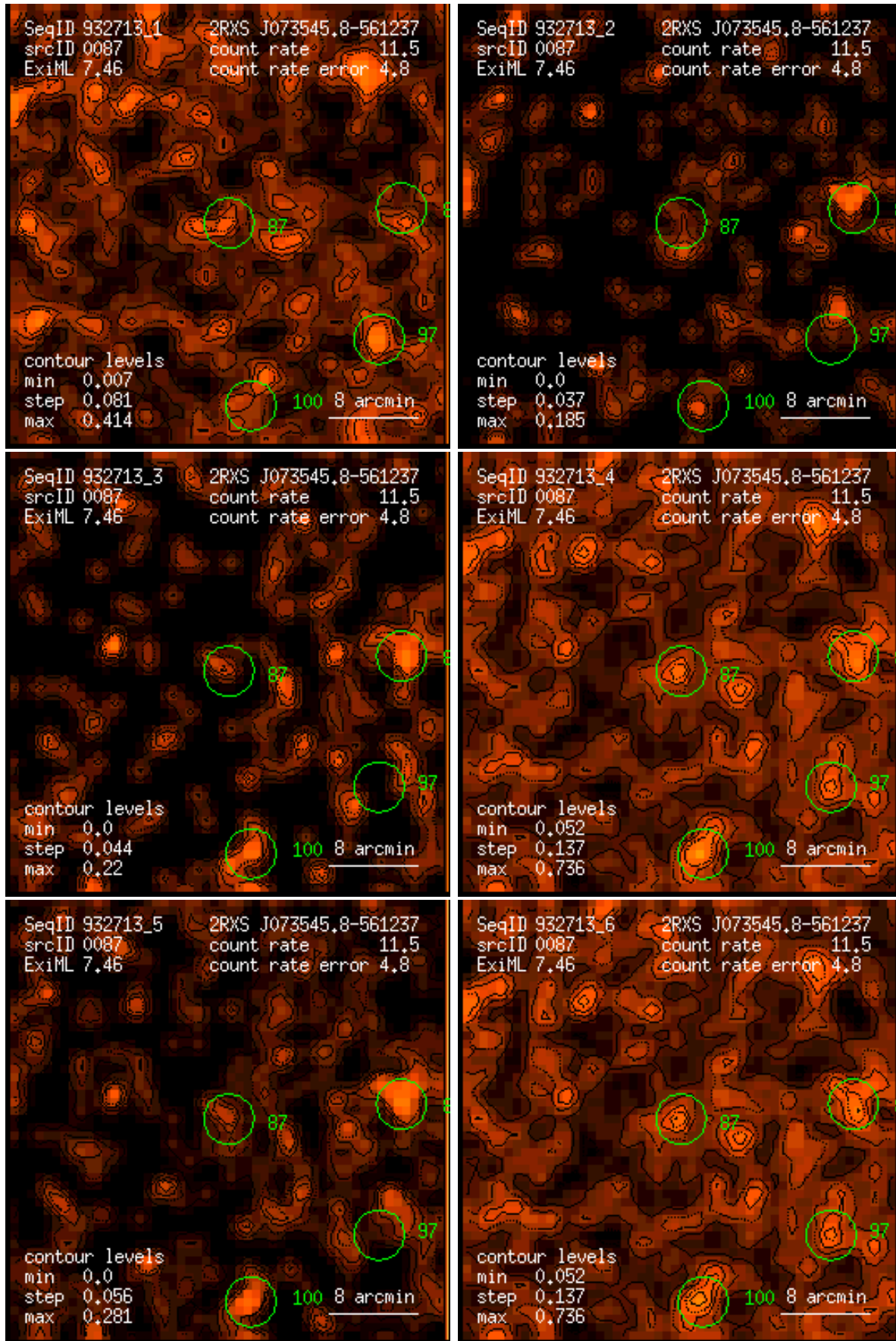
Figure 87: RASS 932713: detection 0087: band rate images, Gaussian filter: (1) PSPC channels 11 – 41, (2) 52 – 90, (3) 91 – 201, (4) 11 – 235, (5) 52 – 201, (6) 11 – 201. Broad band rates in counts/ks. Band rate contour levels in counts/ks/arcmin 2 .
