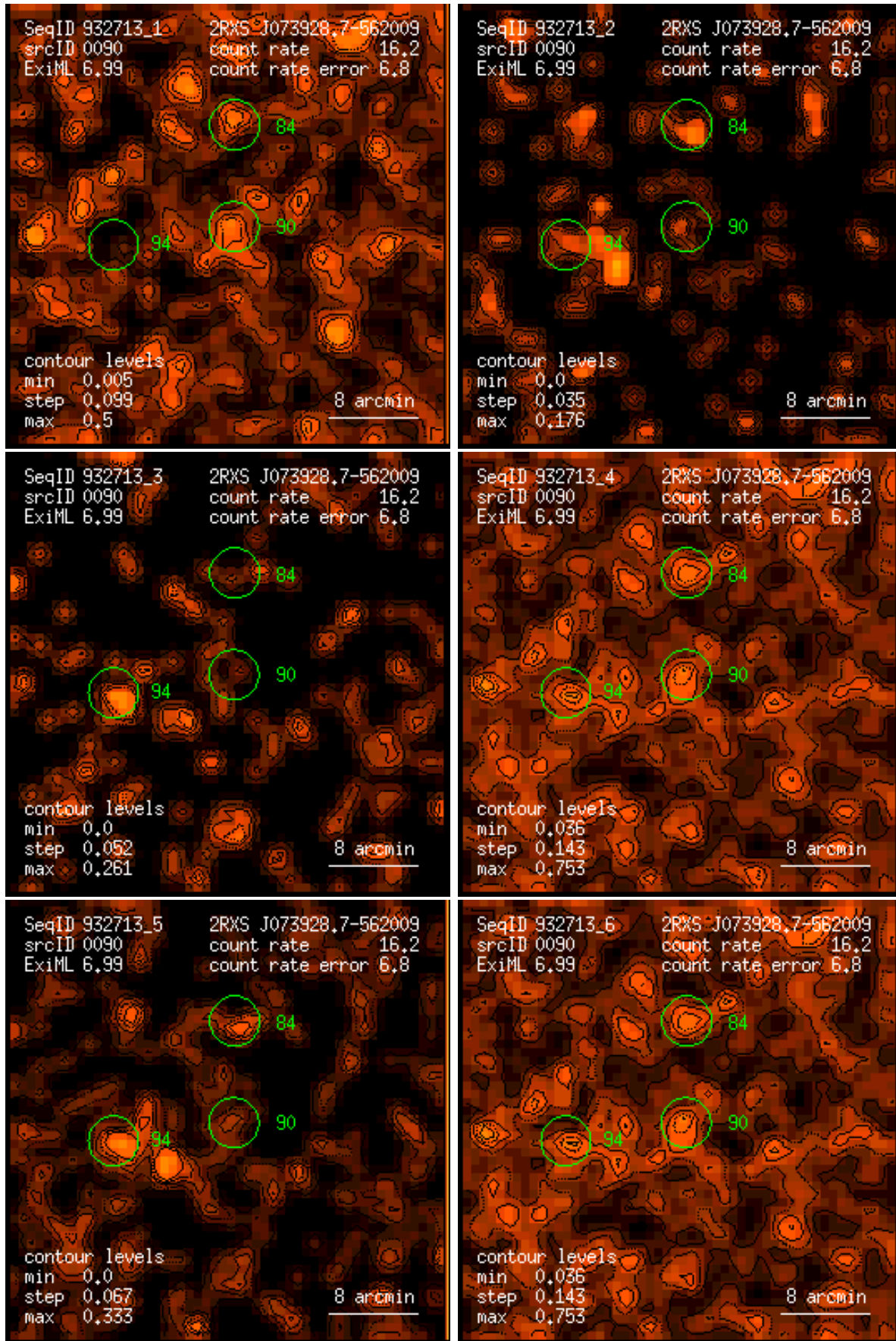
Figure 90: RASS 932713: detection 0090: band rate images, Gaussian filter: (1) PSPC channels 11 – 41, (2) 52 – 90, (3) 91 – 201, (4) 11 – 235, (5) 52 – 201, (6) 11 – 201. Broad band rates in counts/ks. Band rate contour levels in counts/ks/arcmin 2 .
