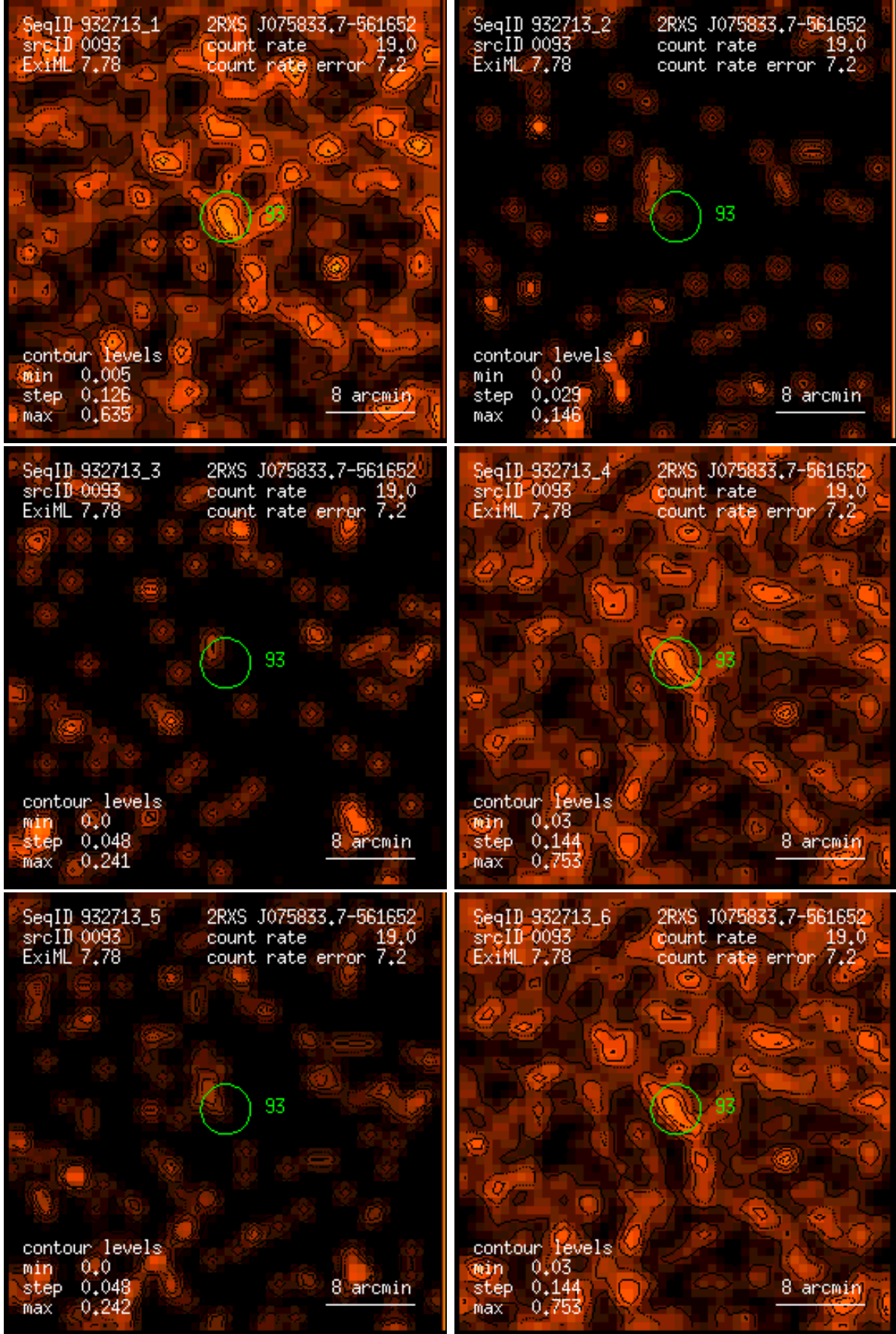
Figure 93: RASS 932713: detection 0093: band rate images, Gaussian filter: (1) PSPC channels 11 – 41, (2) 52 – 90, (3) 91 – 201, (4) 11 – 235, (5) 52 – 201, (6) 11 – 201. Broad band rates in counts/ks. Band rate contour levels in counts/ks/arcmin 2 .
