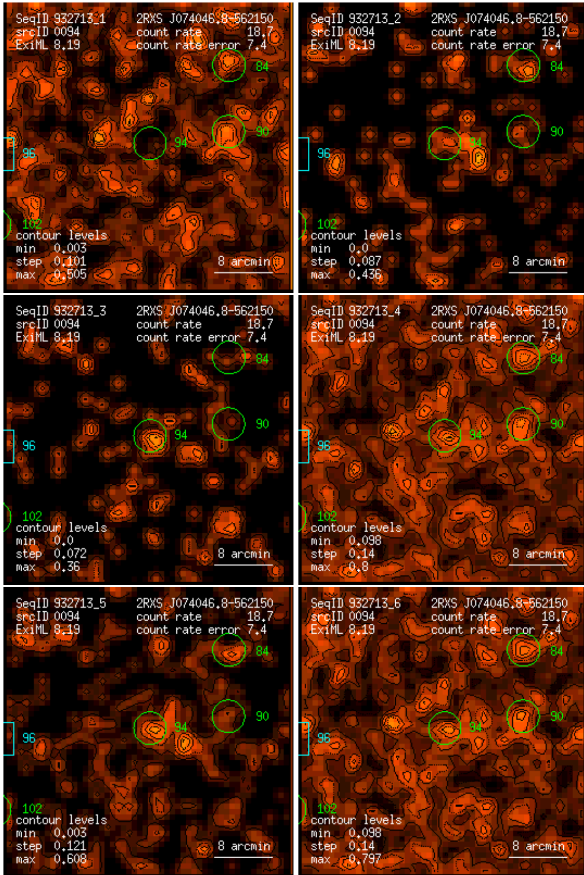
Figure 94: RASS 932713: detection 0094: band rate images, Gaussian filter: (1) PSPC channels 11 – 41, (2) 52 – 90, (3) 91 – 201, (4) 11 – 235, (5) 52 – 201, (6) 11 – 201. Broad band rates in counts/ks. Band rate contour levels in counts/ks/arcmin 2 .
