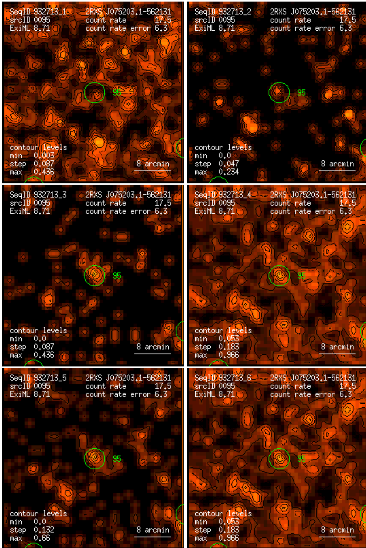
Figure 95: RASS 932713: detection 0095: band rate images, Gaussian filter: (1) PSPC channels 11 – 41, (2) 52 – 90, (3) 91 – 201, (4) 11 – 235, (5) 52 – 201, (6) 11 – 201. Broad band rates in counts/ks. Band rate contour levels in counts/ks/arcmin 2 .
