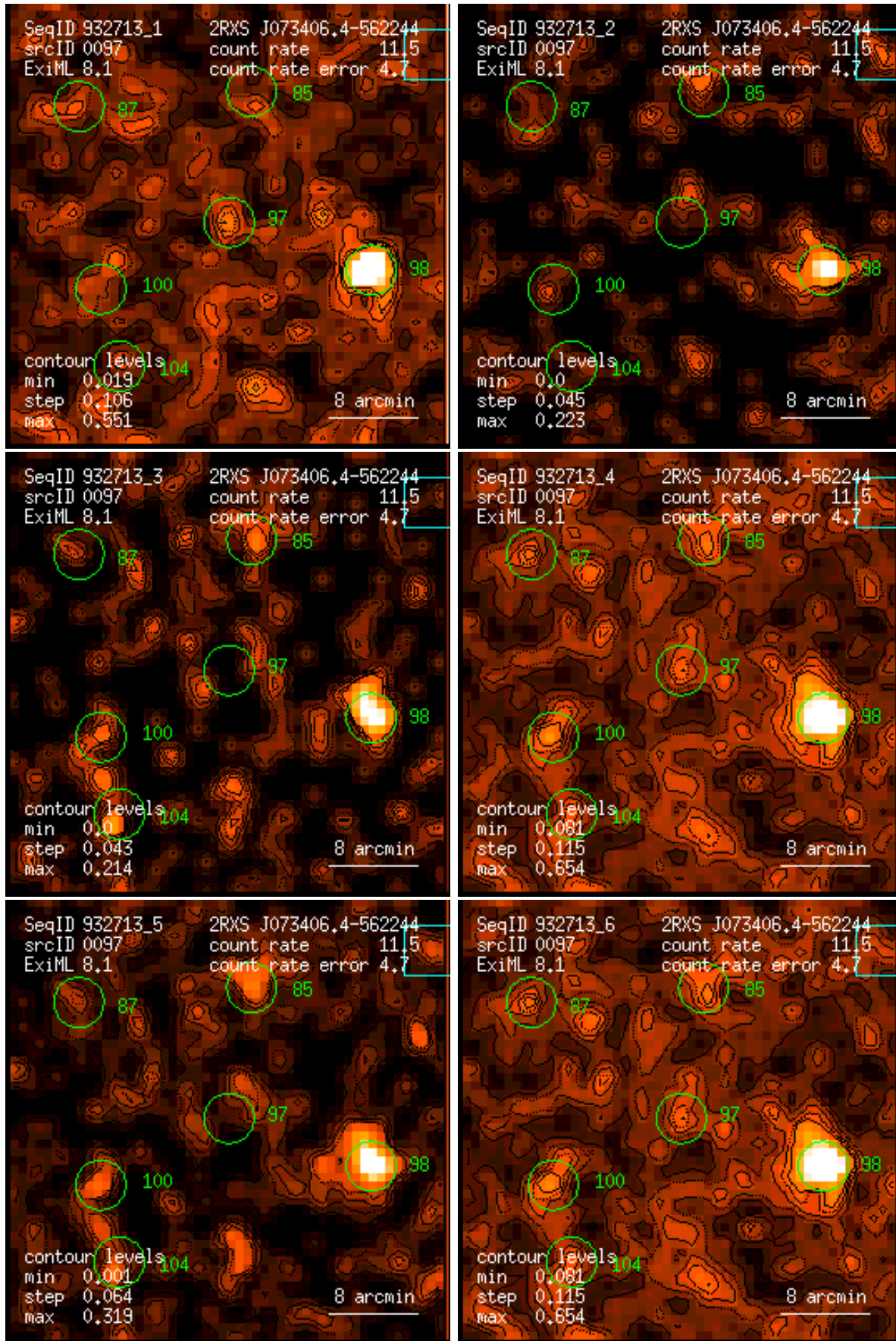
Figure 97: RASS 932713: detection 0097: band rate images, Gaussian filter: (1) PSPC channels 11 – 41, (2) 52 – 90, (3) 91 – 201, (4) 11 – 235, (5) 52 – 201, (6) 11 – 201. Broad band rates in counts/ks. Band rate contour levels in counts/ks/arcmin 2 .
