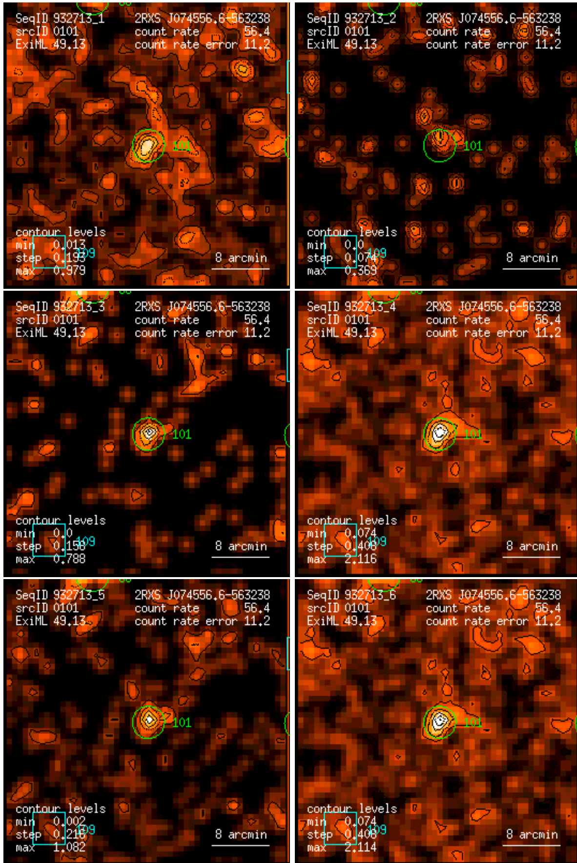
Figure 101: RASS 932713: detection 0101: band rate images, Gaussian filter: (1) PSPC channels 11 – 41, (2) 52 – 90, (3) 91 – 201, (4) 11 – 235, (5) 52 – 201, (6) 11 – 201. Broad band rates in counts/ks. Band rate contour levels in counts/ks/arcmin 2 .
