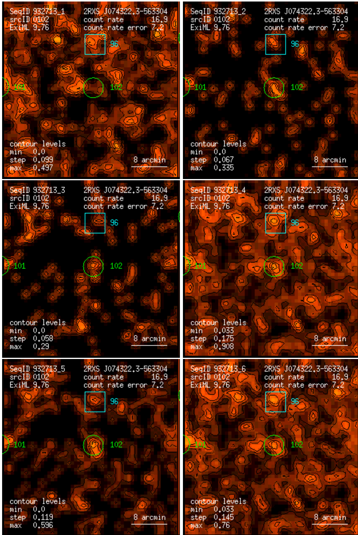
Figure 102: RASS 932713: detection 0102: band rate images, Gaussian filter: (1) PSPC channels 11 – 41, (2) 52 – 90, (3) 91 – 201, (4) 11 – 235, (5) 52 – 201, (6) 11 – 201. Broad band rates in counts/ks. Band rate contour levels in counts/ks/arcmin 2 .
