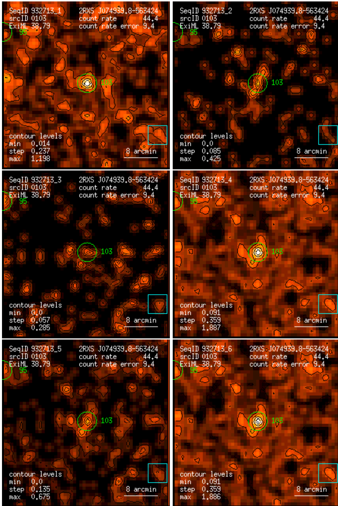
Figure 103: RASS 932713: detection 0103: band rate images, Gaussian filter: (1) PSPC channels 11 – 41, (2) 52 – 90, (3) 91 – 201, (4) 11 – 235, (5) 52 – 201, (6) 11 – 201. Broad band rates in counts/ks. Band rate contour levels in counts/ks/arcmin 2 .
