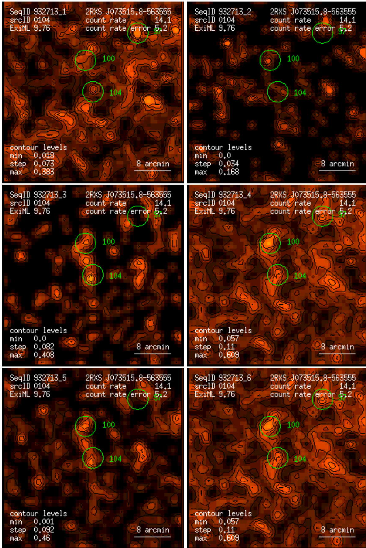
Figure 104: RASS 932713: detection 0104: band rate images, Gaussian filter: (1) PSPC channels 11 – 41, (2) 52 – 90, (3) 91 – 201, (4) 11 – 235, (5) 52 – 201, (6) 11 – 201. Broad band rates in counts/ks. Band rate contour levels in counts/ks/arcmin 2 .
