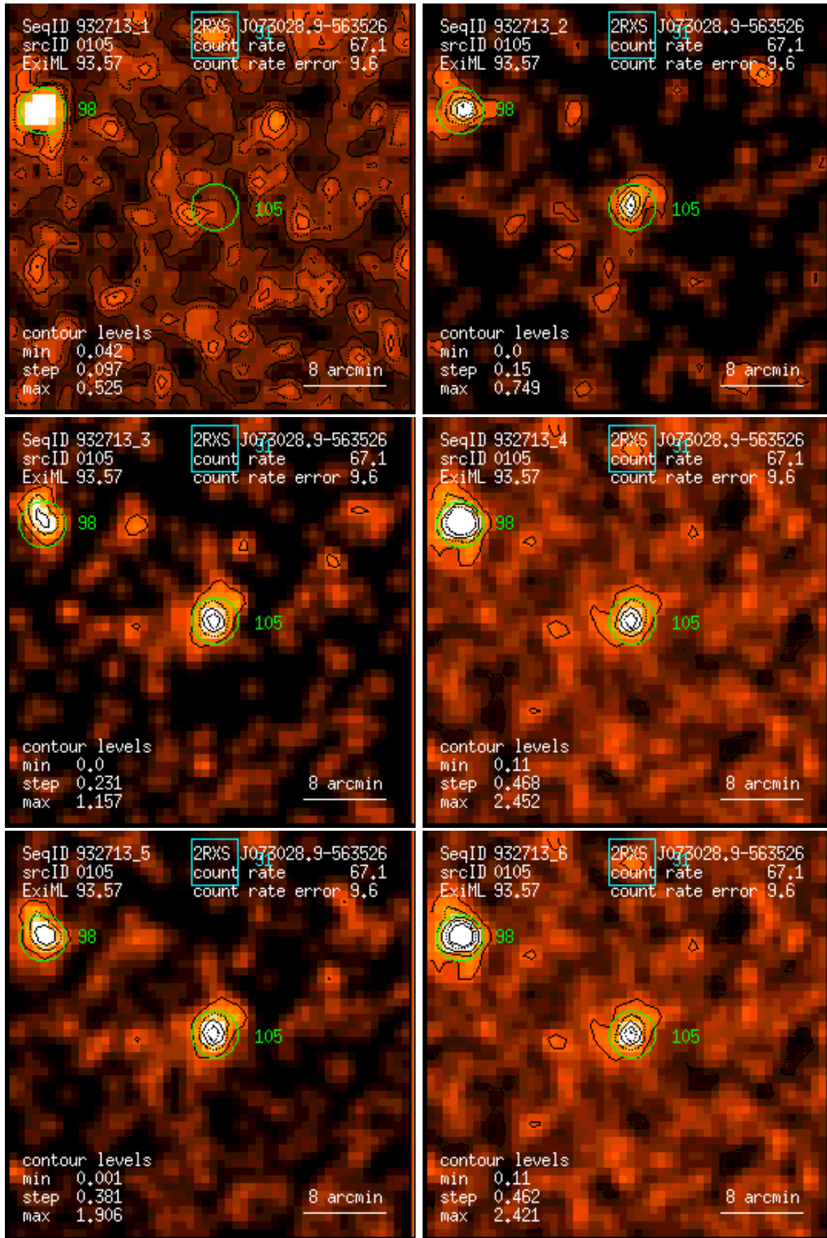
Figure 105: RASS 932713: detection 0105: band rate images, Gaussian filter: (1) PSPC channels 11 – 41, (2) 52 – 90, (3) 91 – 201, (4) 11 – 235, (5) 52 – 201, (6) 11 – 201. Broad band rates in counts/ks. Band rate contour levels in counts/ks/arcmin 2 .
