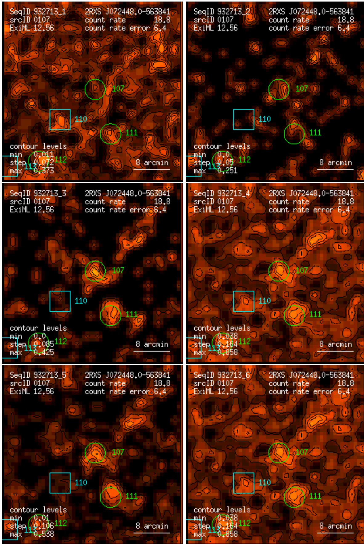
Figure 107: RASS 932713: detection 0107: band rate images, Gaussian filter: (1) PSPC channels 11 – 41, (2) 52 – 90, (3) 91 – 201, (4) 11 – 235, (5) 52 – 201, (6) 11 – 201. Broad band rates in counts/ks. Band rate contour levels in counts/ks/arcmin 2 .
