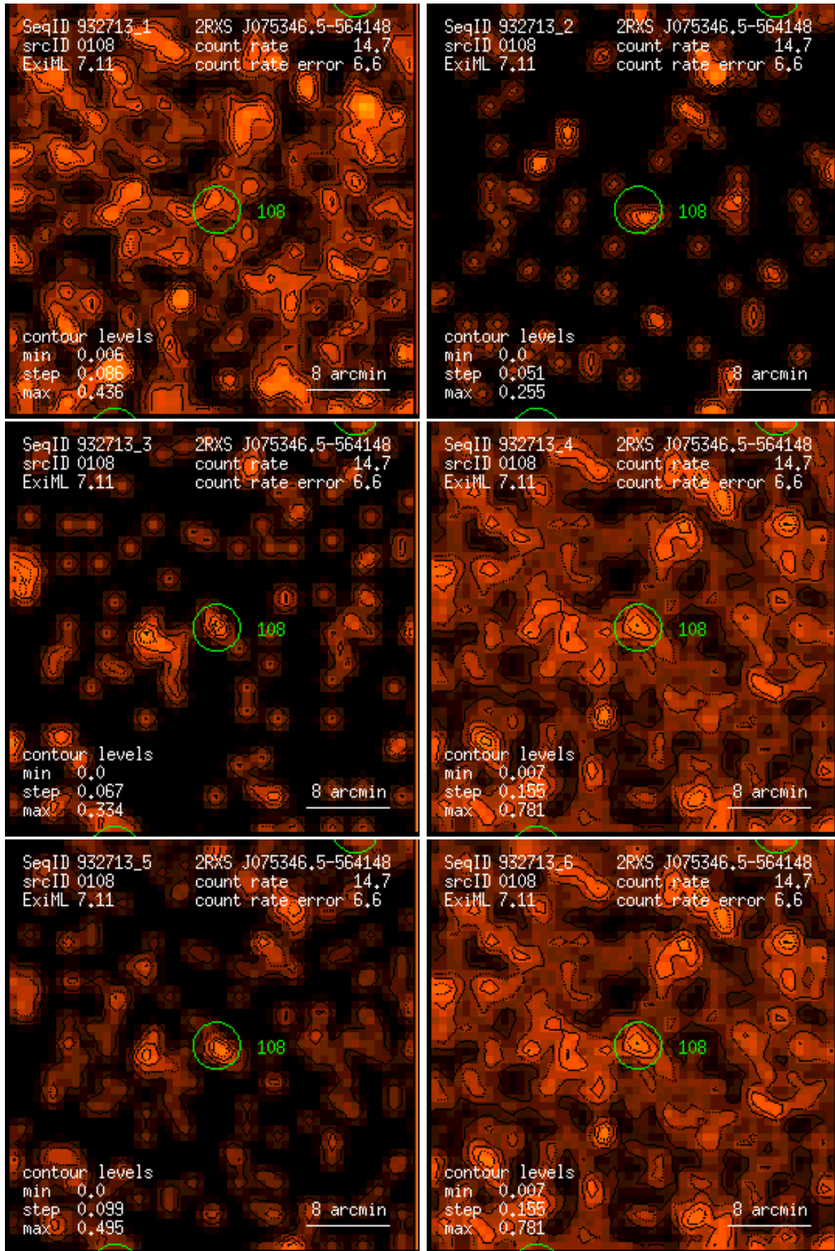
Figure 108: RASS 932713: detection 0108: band rate images, Gaussian filter: (1) PSPC channels 11 – 41, (2) 52 – 90, (3) 91 – 201, (4) 11 – 235, (5) 52 – 201, (6) 11 – 201. Broad band rates in counts/ks. Band rate contour levels in counts/ks/arcmin 2 .
