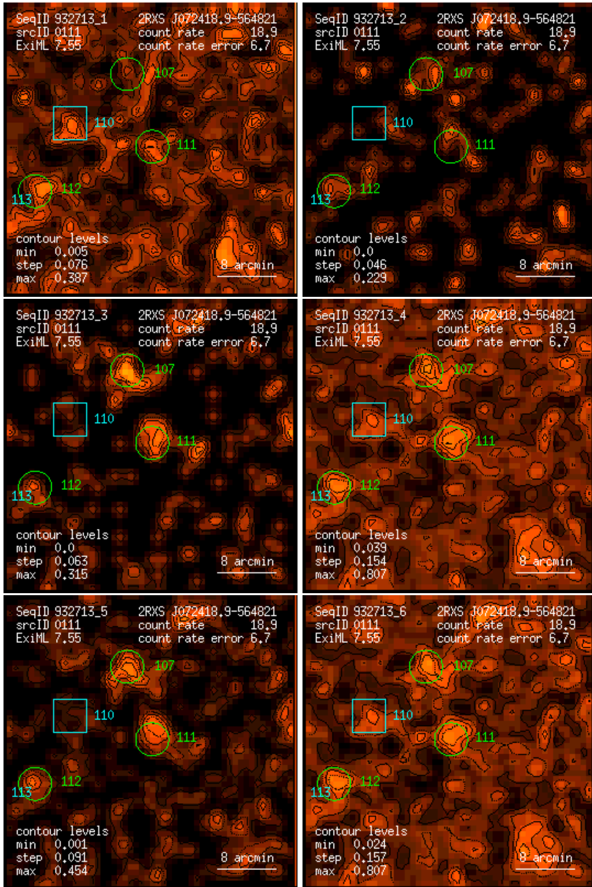
Figure 111: RASS 932713: detection 0111: band rate images, Gaussian filter: (1) PSPC channels 11 – 41, (2) 52 – 90, (3) 91 – 201, (4) 11 – 235, (5) 52 – 201, (6) 11 – 201. Broad band rates in counts/ks. Band rate contour levels in counts/ks/arcmin 2 .
