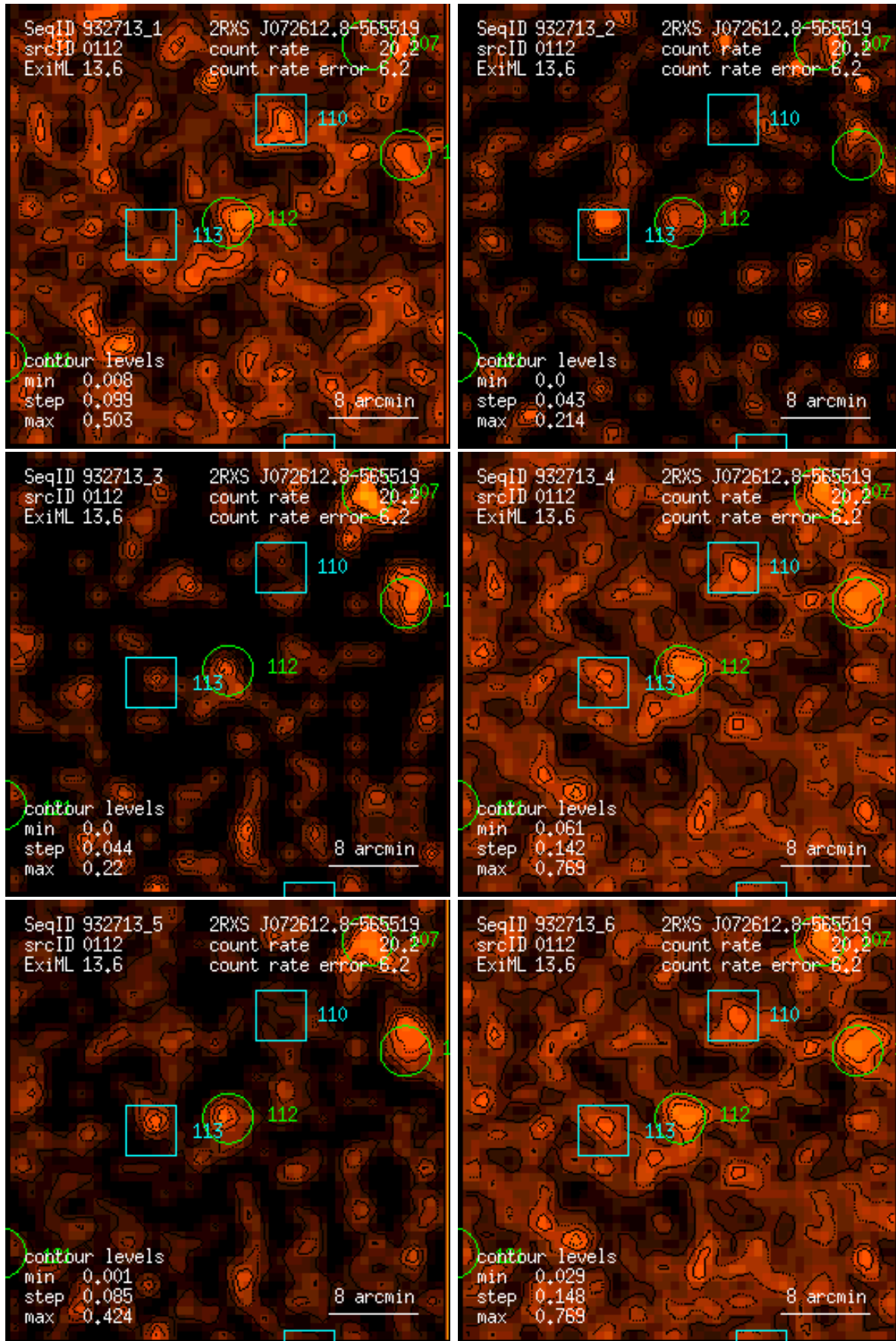
Figure 112: RASS 932713: detection 0112: band rate images, Gaussian filter: (1) PSPC channels 11 – 41, (2) 52 – 90, (3) 91 – 201, (4) 11 – 235, (5) 52 – 201, (6) 11 – 201. Broad band rates in counts/ks. Band rate contour levels in counts/ks/arcmin 2 .
