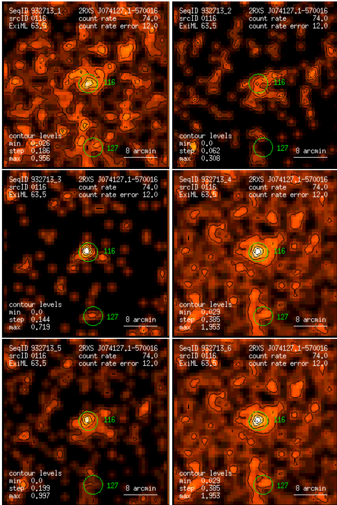
Figure 116: RASS 932713: detection 0116: band rate images, Gaussian filter: (1) PSPC channels 11 – 41, (2) 52 – 90, (3) 91 – 201, (4) 11 – 235, (5) 52 – 201, (6) 11 – 201. Broad band rates in counts/ks. Band rate contour levels in counts/ks/arcmin 2 .
