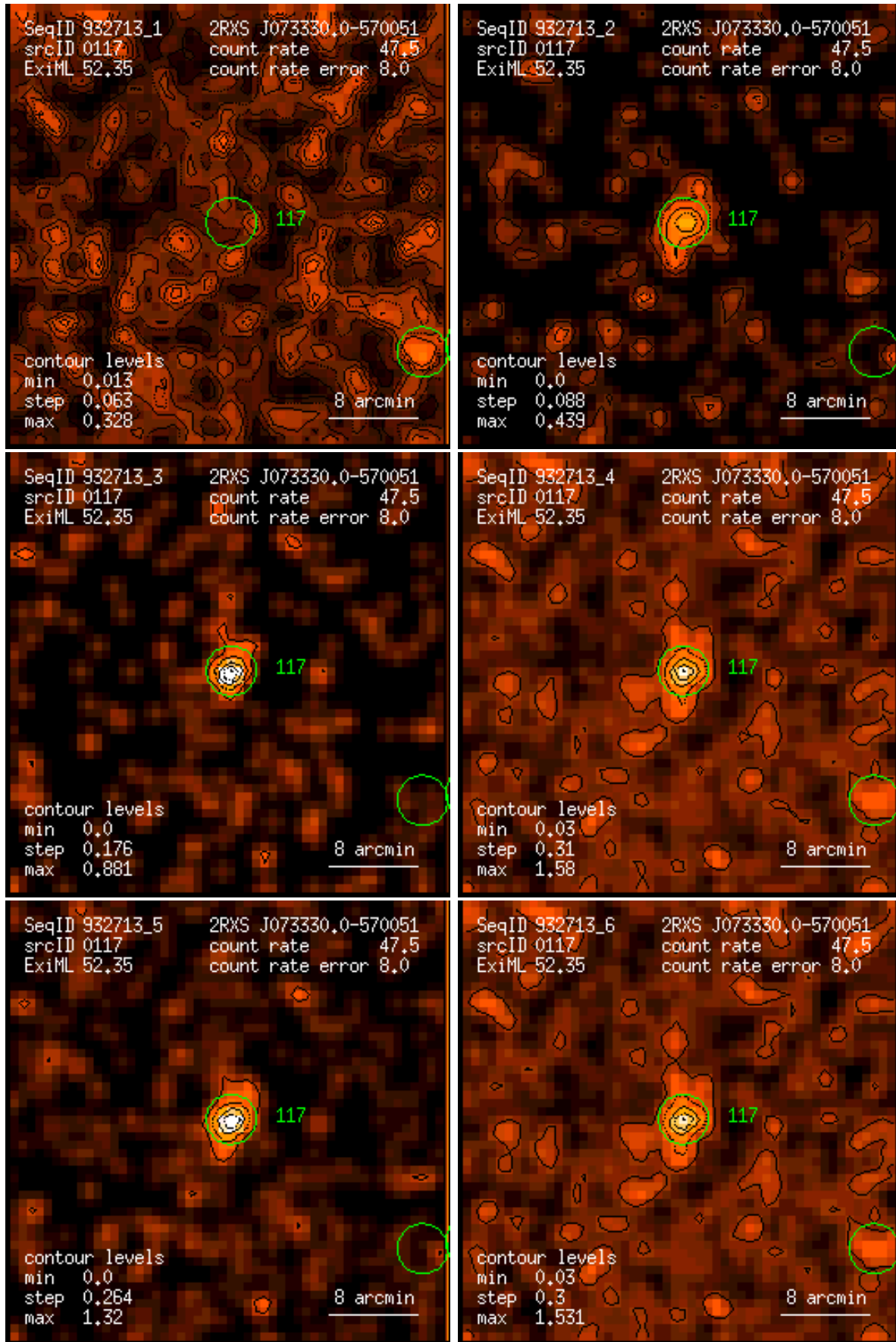
Figure 117: RASS 932713: detection 0117: band rate images, Gaussian filter: (1) PSPC channels 11 – 41, (2) 52 – 90, (3) 91 – 201, (4) 11 – 235, (5) 52 – 201, (6) 11 – 201. Broad band rates in counts/ks. Band rate contour levels in counts/ks/arcmin 2 .
