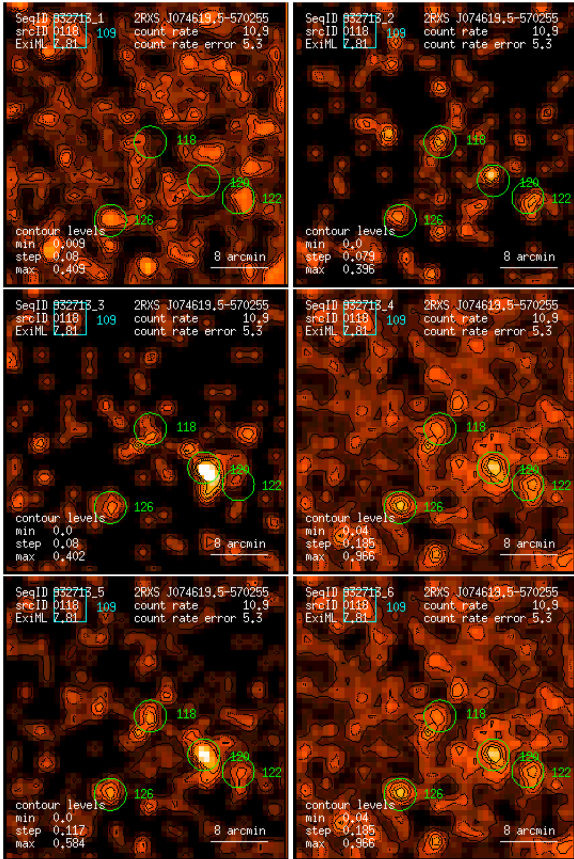
Figure 118: RASS 932713: detection 0118: band rate images, Gaussian filter: (1) PSPC channels 11 – 41, (2) 52 – 90, (3) 91 – 201, (4) 11 – 235, (5) 52 – 201, (6) 11 – 201. Broad band rates in counts/ks. Band rate contour levels in counts/ks/arcmin 2 .
