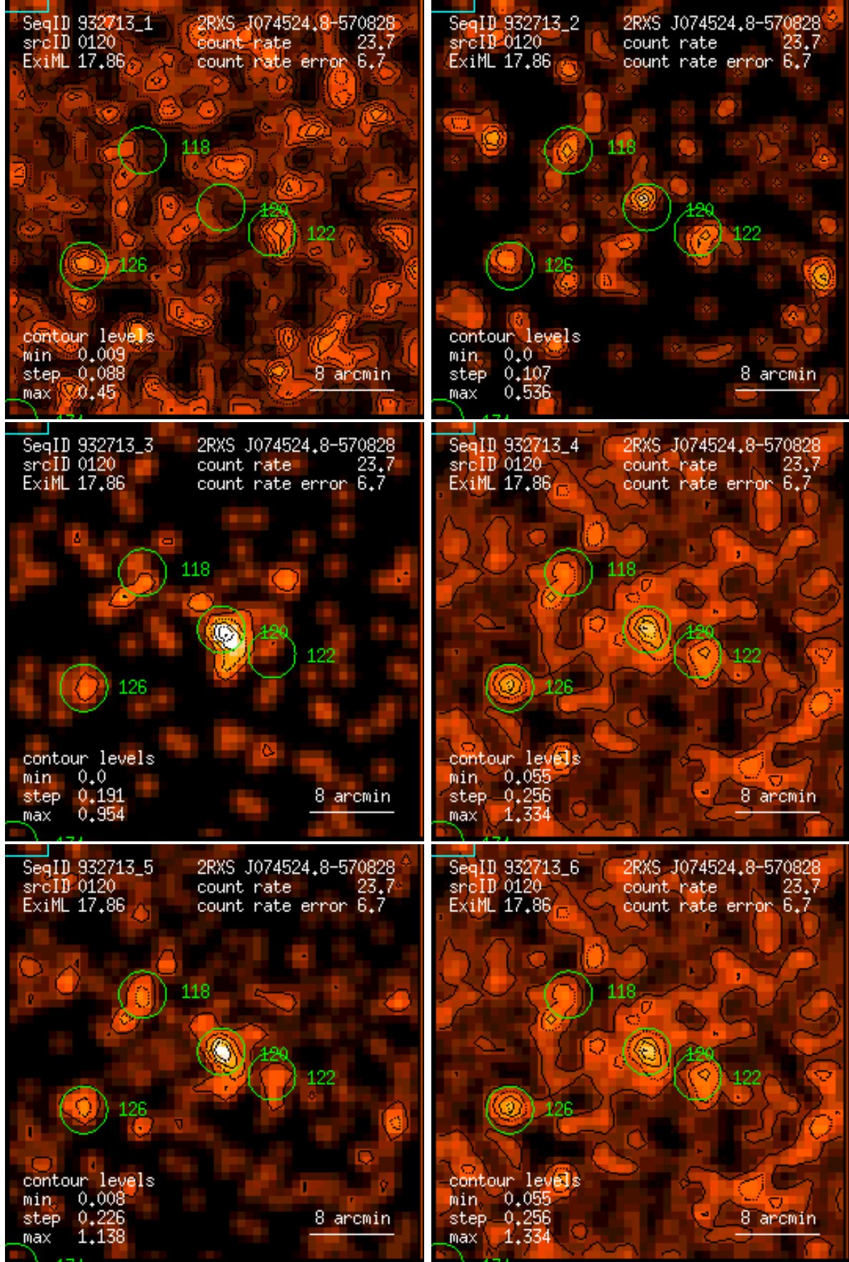
Figure 120: RASS 932713: detection 0120: band rate images, Gaussian filter: (1) PSPC channels 11 – 41, (2) 52 – 90, (3) 91 – 201, (4) 11 – 235, (5) 52 – 201, (6) 11 – 201. Broad band rates in counts/ks. Band rate contour levels in counts/ks/arcmin 2 .
