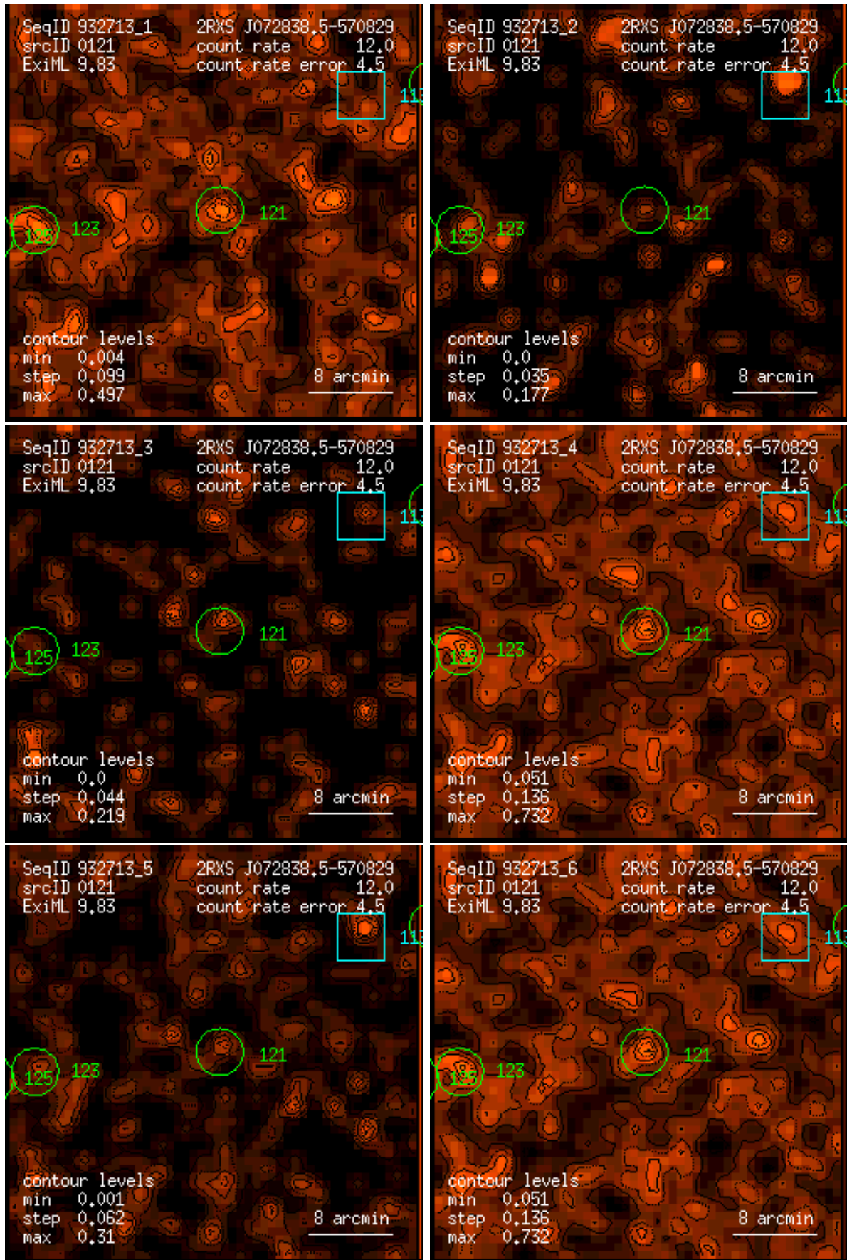
Figure 121: RASS 932713: detection 0121: band rate images, Gaussian filter: (1) PSPC channels 11 – 41, (2) 52 – 90, (3) 91 – 201, (4) 11 – 235, (5) 52 – 201, (6) 11 – 201. Broad band rates in counts/ks. Band rate contour levels in counts/ks/arcmin 2 .
