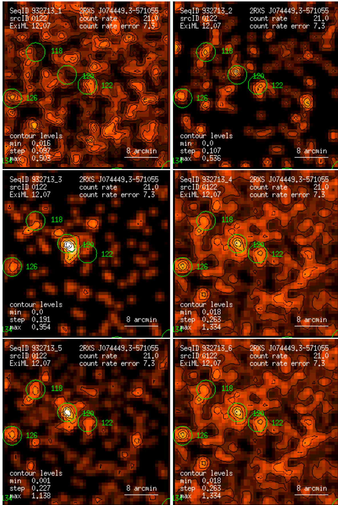
Figure 122: RASS 932713: detection 0122: band rate images, Gaussian filter: (1) PSPC channels 11 – 41, (2) 52 – 90, (3) 91 – 201, (4) 11 – 235, (5) 52 – 201, (6) 11 – 201. Broad band rates in counts/ks. Band rate contour levels in counts/ks/arcmin 2 .
