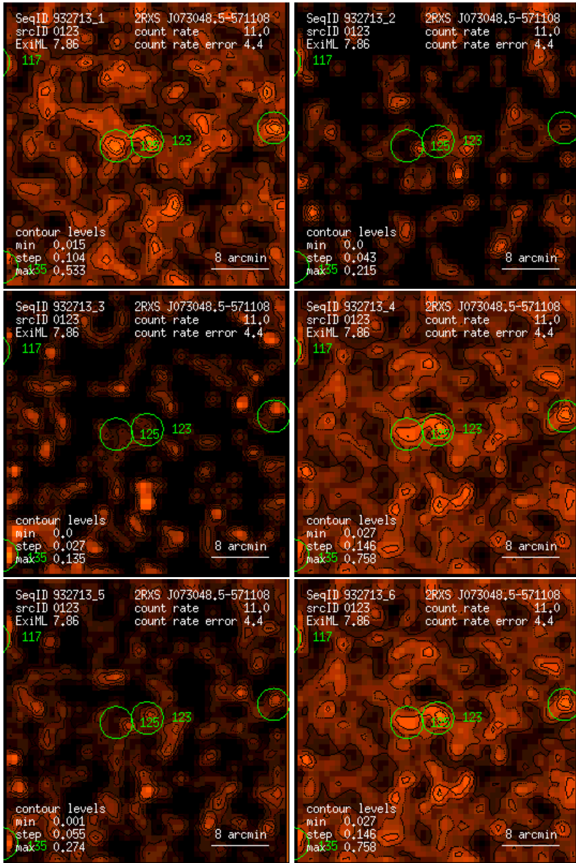
Figure 123: RASS 932713: detection 0123: band rate images, Gaussian filter: (1) PSPC channels 11 – 41, (2) 52 – 90, (3) 91 – 201, (4) 11 – 235, (5) 52 – 201, (6) 11 – 201. Broad band rates in counts/ks. Band rate contour levels in counts/ks/arcmin 2 .
