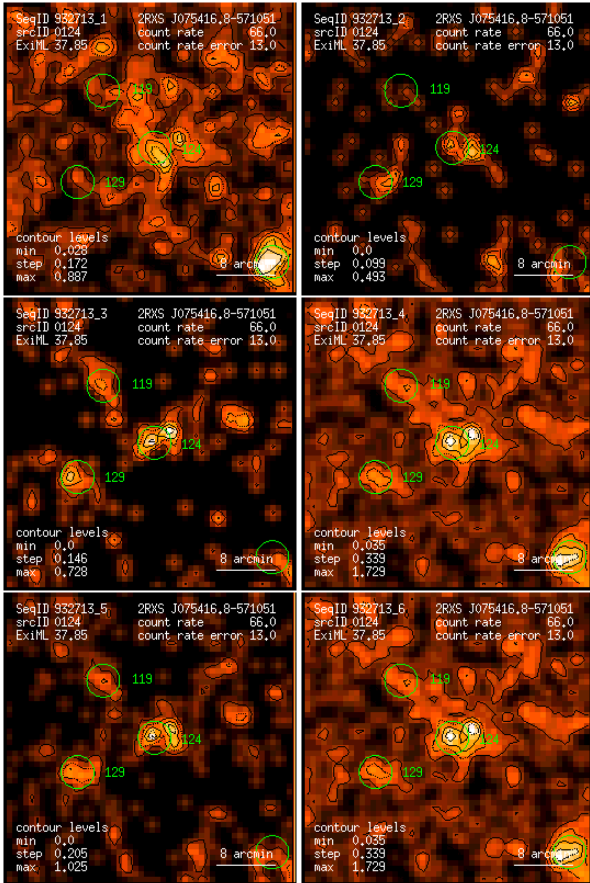
Figure 124: RASS 932713: detection 0124: band rate images, Gaussian filter: (1) PSPC channels 11 – 41, (2) 52 – 90, (3) 91 – 201, (4) 11 – 235, (5) 52 – 201, (6) 11 – 201. Broad band rates in counts/ks. Band rate contour levels in counts/ks/arcmin 2 .
