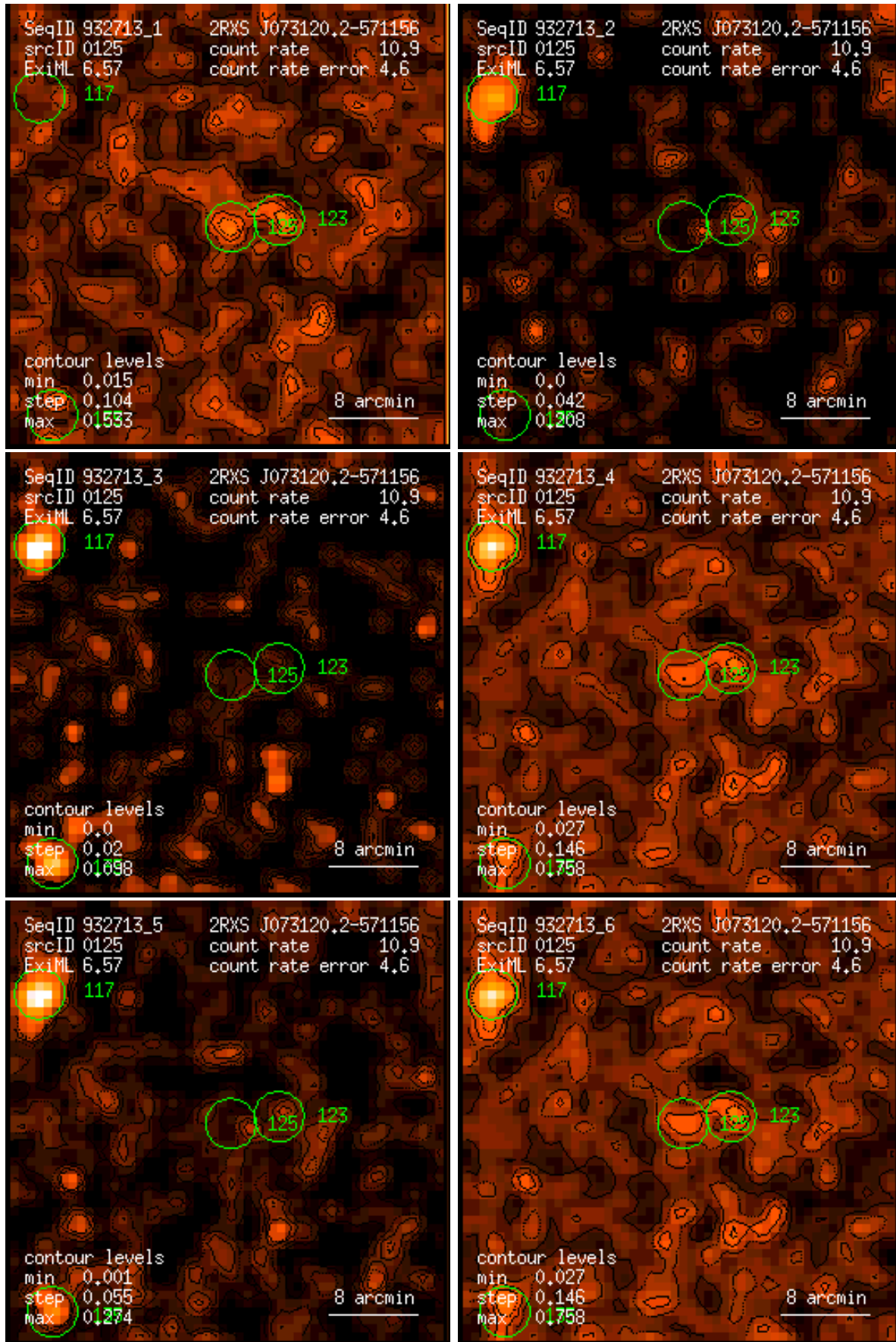
Figure 125: RASS 932713: detection 0125: band rate images, Gaussian filter: (1) PSPC channels 11 – 41, (2) 52 – 90, (3) 91 – 201, (4) 11 – 235, (5) 52 – 201, (6) 11 – 201. Broad band rates in counts/ks. Band rate contour levels in counts/ks/arcmin 2 .
