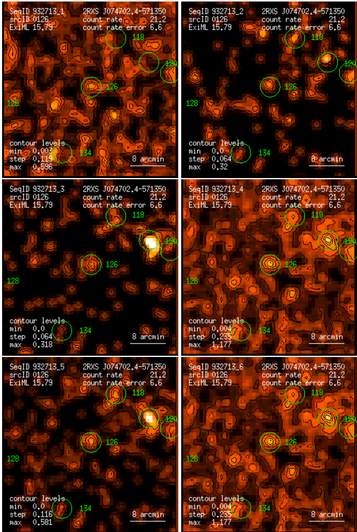
Figure 126: RASS 932713: detection 0126: band rate images, Gaussian filter: (1) PSPC channels 11 – 41, (2) 52 – 90, (3) 91 – 201, (4) 11 – 235, (5) 52 – 201, (6) 11 – 201. Broad band rates in counts/ks. Band rate contour levels in counts/ks/arcmin 2 .
