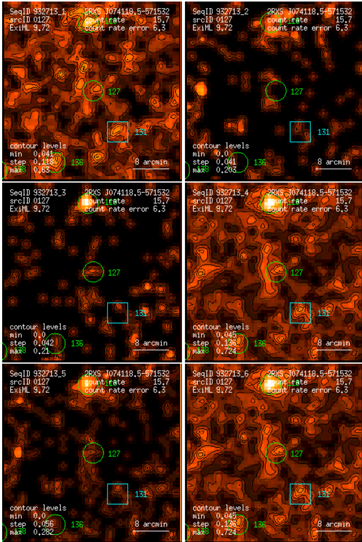
Figure 127: RASS 932713: detection 0127: band rate images, Gaussian filter: (1) PSPC channels 11 – 41, (2) 52 – 90, (3) 91 – 201, (4) 11 – 235, (5) 52 – 201, (6) 11 – 201. Broad band rates in counts/ks. Band rate contour levels in counts/ks/arcmin 2 .
