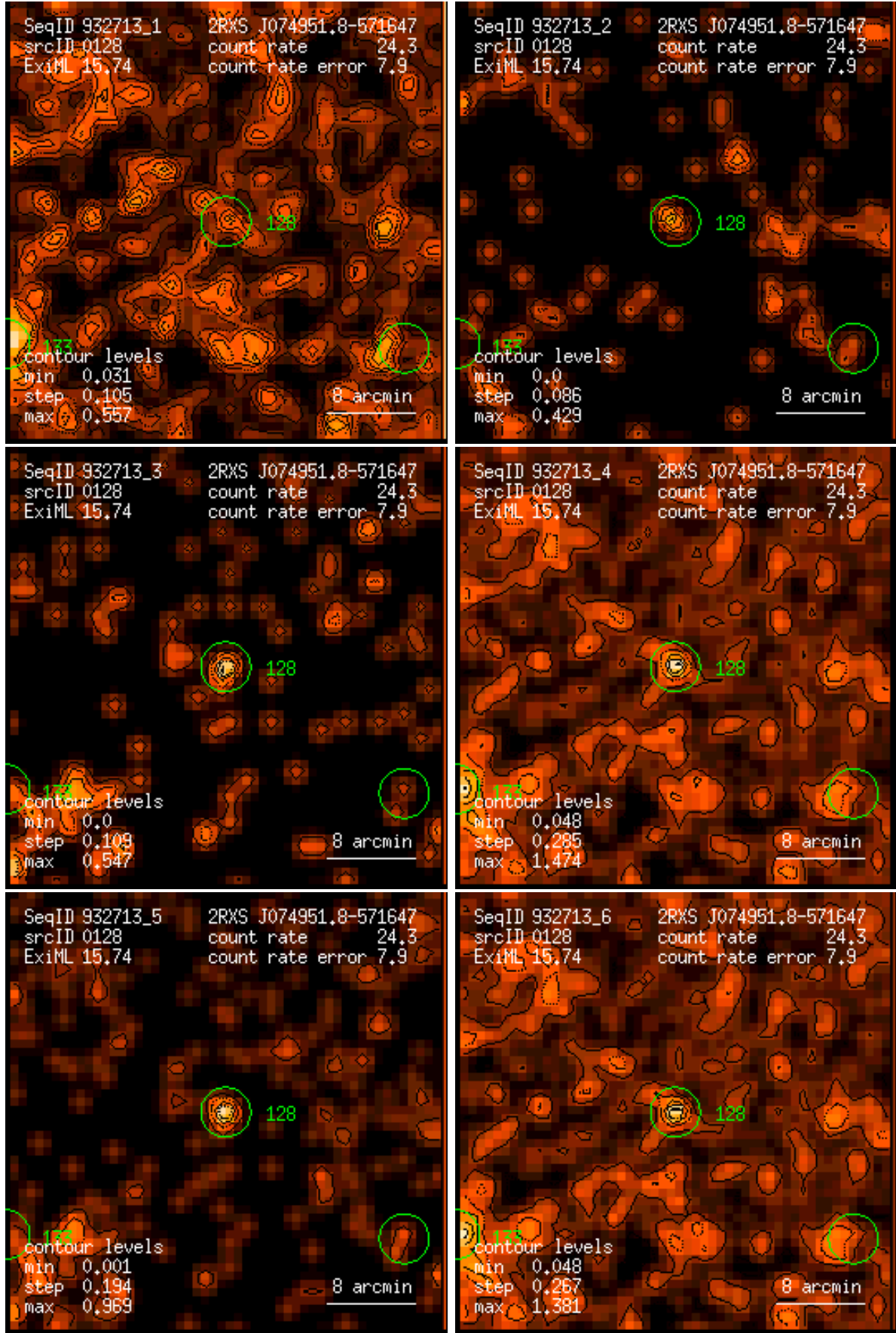
Figure 128: RASS 932713: detection 0128: band rate images, Gaussian filter: (1) PSPC channels 11 – 41, (2) 52 – 90, (3) 91 – 201, (4) 11 – 235, (5) 52 – 201, (6) 11 – 201. Broad band rates in counts/ks. Band rate contour levels in counts/ks/arcmin 2 .
