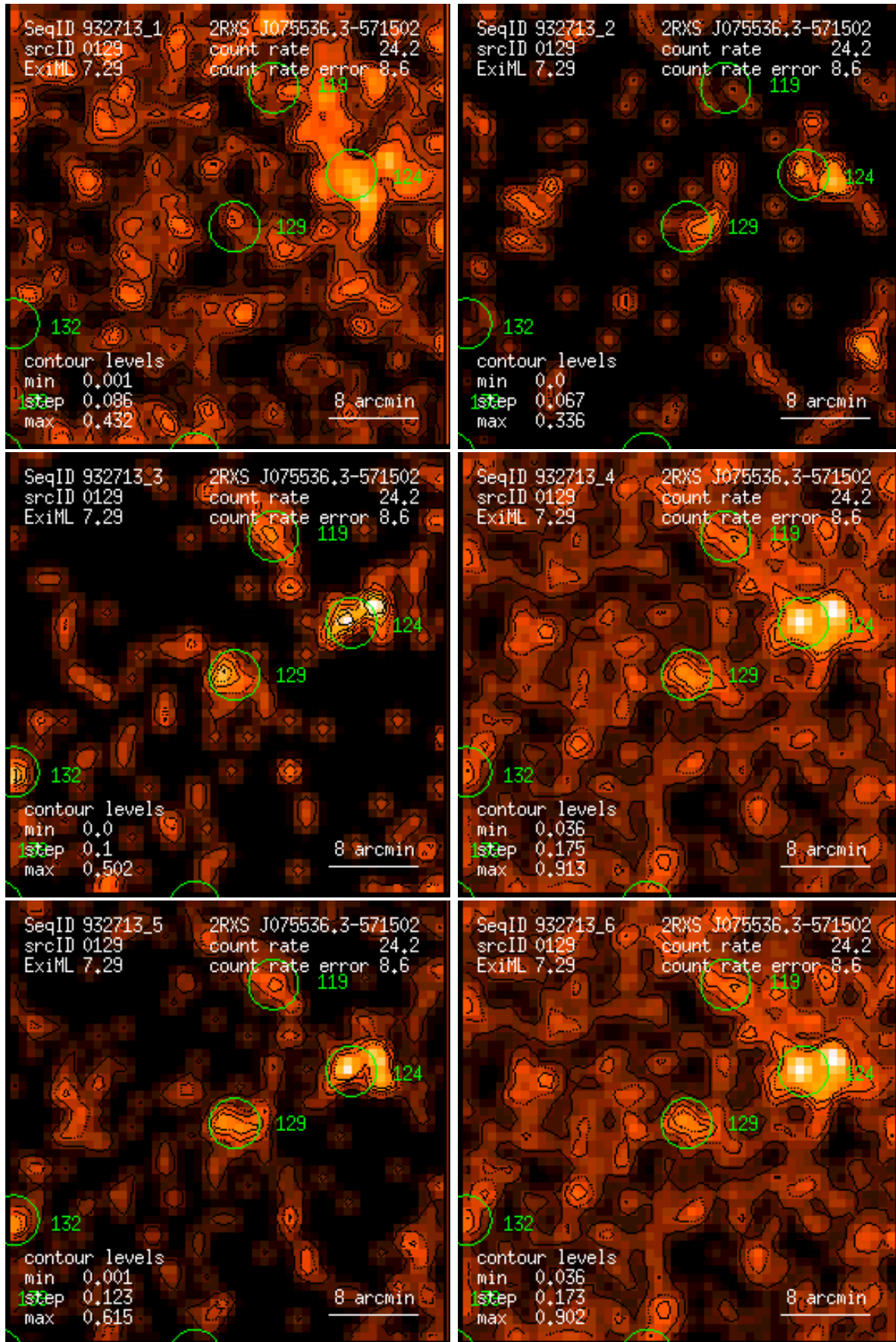
Figure 129: RASS 932713: detection 0129: band rate images, Gaussian filter: (1) PSPC channels 11 – 41, (2) 52 – 90, (3) 91 – 201, (4) 11 – 235, (5) 52 – 201, (6) 11 – 201. Broad band rates in counts/ks. Band rate contour levels in counts/ks/arcmin 2 .
