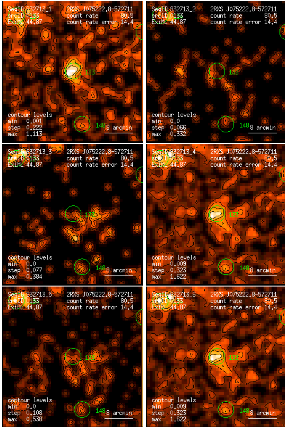
Figure 133: RASS 932713: detection 0133: band rate images, Gaussian filter: (1) PSPC channels 11 – 41, (2) 52 – 90, (3) 91 – 201, (4) 11 – 235, (5) 52 – 201, (6) 11 – 201. Broad band rates in counts/ks. Band rate contour levels in counts/ks/arcmin 2 .
