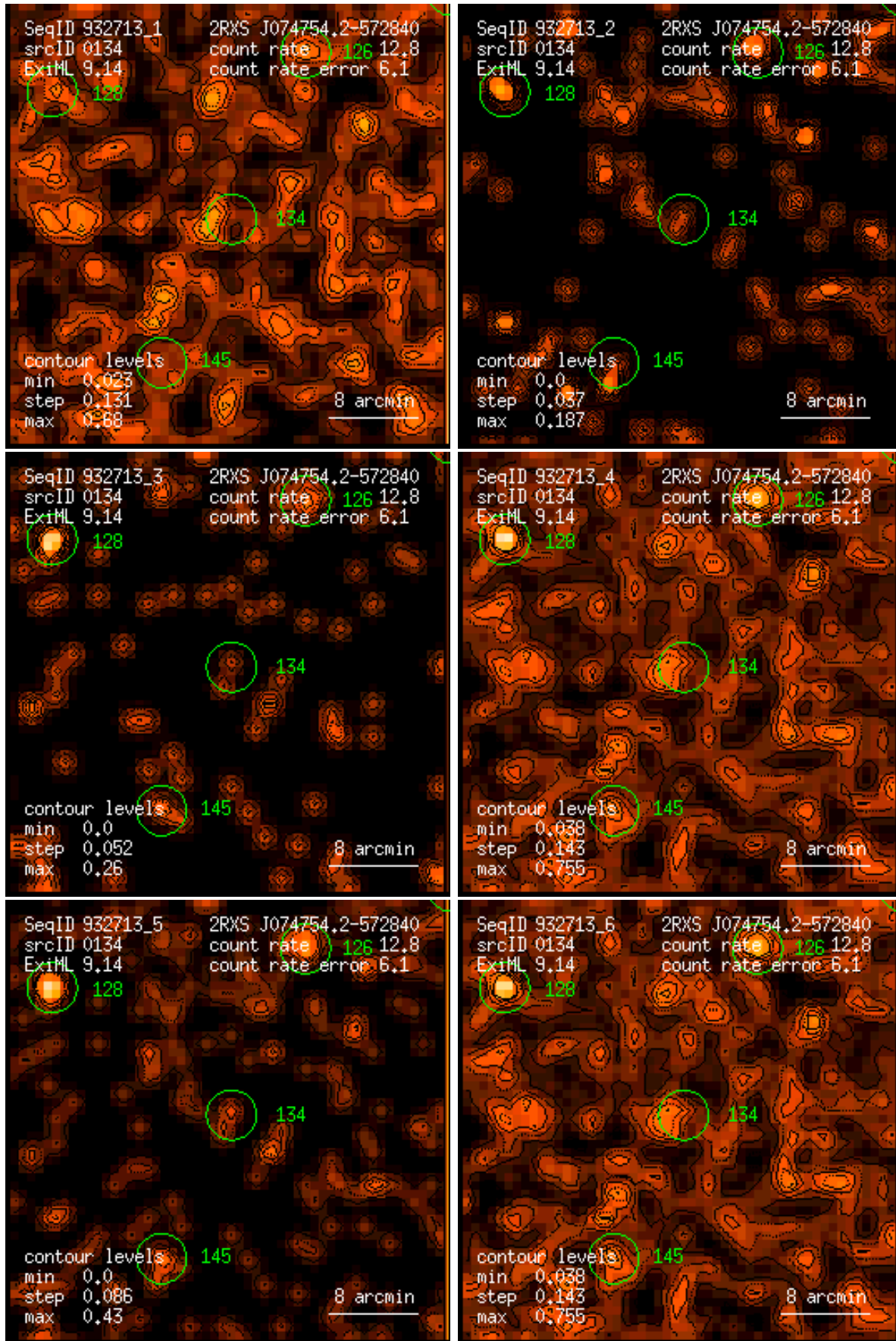
Figure 134: RASS 932713: detection 0134: band rate images, Gaussian filter: (1) PSPC channels 11 – 41, (2) 52 – 90, (3) 91 – 201, (4) 11 – 235, (5) 52 – 201, (6) 11 – 201. Broad band rates in counts/ks. Band rate contour levels in counts/ks/arcmin 2 .
