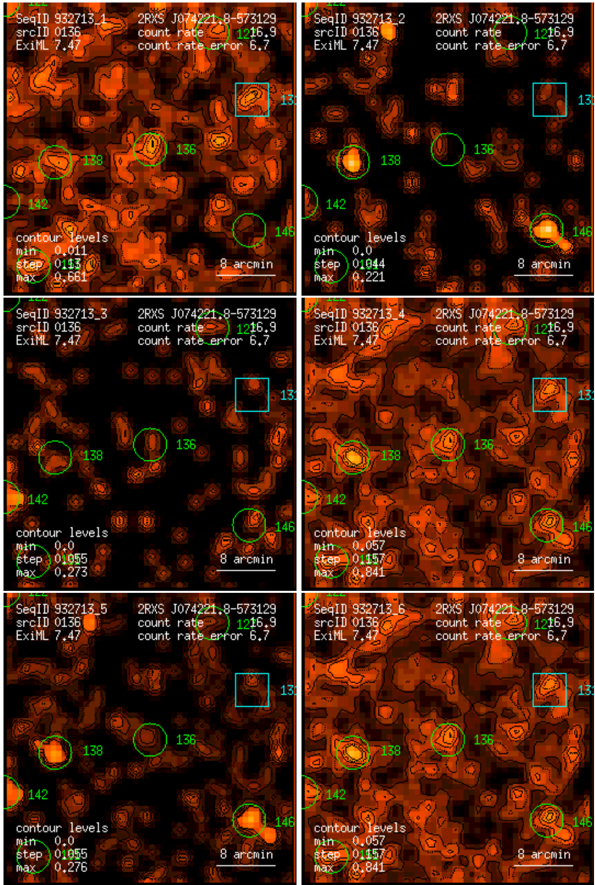
Figure 136: RASS 932713: detection 0136: band rate images, Gaussian filter: (1) PSPC channels 11 – 41, (2) 52 – 90, (3) 91 – 201, (4) 11 – 235, (5) 52 – 201, (6) 11 – 201. Broad band rates in counts/ks. Band rate contour levels in counts/ks/arcmin 2 .
