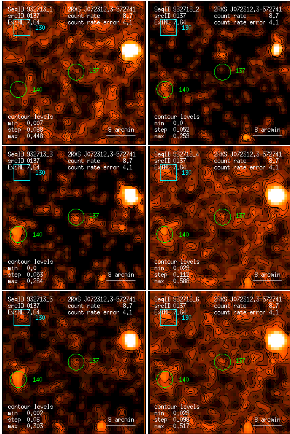
Figure 137: RASS 932713: detection 0137: band rate images, Gaussian filter: (1) PSPC channels 11 – 41, (2) 52 – 90, (3) 91 – 201, (4) 11 – 235, (5) 52 – 201, (6) 11 – 201. Broad band rates in counts/ks. Band rate contour levels in counts/ks/arcmin 2 .
